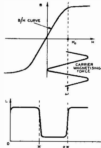
FIG. 2.—B/H CURVE FOR THE INDUCTOR, AND SWITCHING OF INDUCTANCE BY CARRIER MAGNETISING FORCE.
