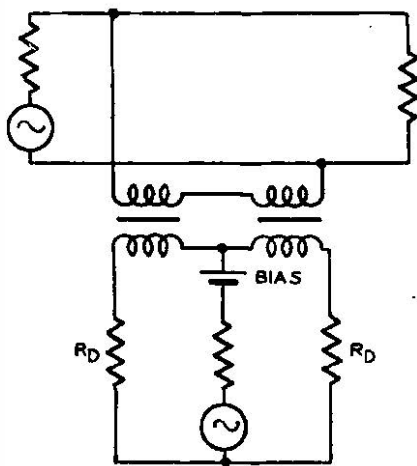
FIG. 4.—BALANCED MODULATOR.
