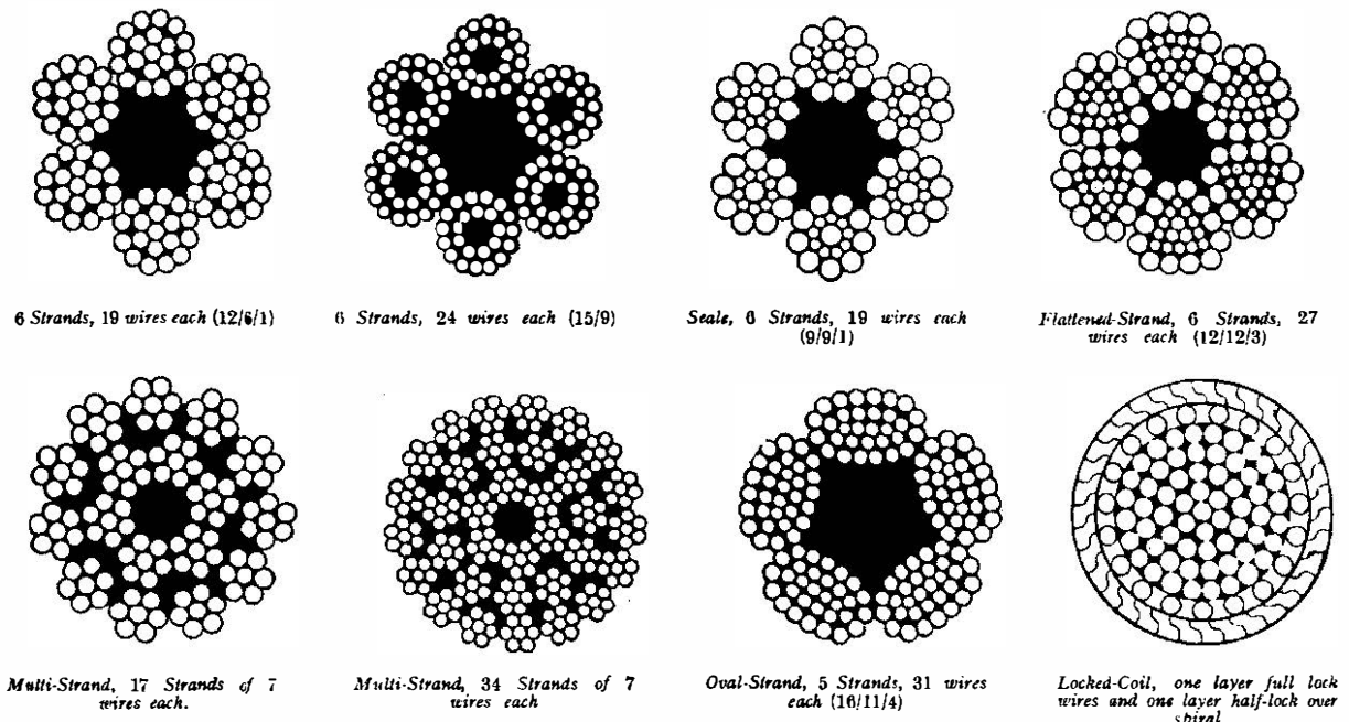
FIG. 8.—TYPICAL ROPE CONSTRUCTIONS.
