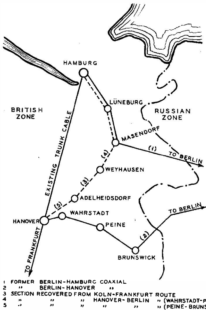
FIG. 1.—ROUTES TAKEN BY CABLES IN THE BRITISH ZONE OF GERMANY.
