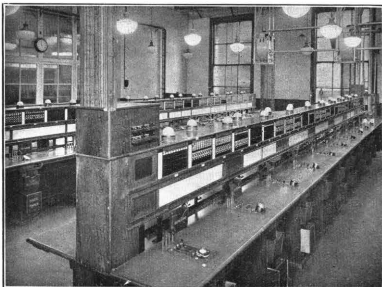
FIG. 1.—THE PHONOGRAM SWITCHROOM AT NEWCASTLE, EQUIPPED WITH DOUBLE-TIER ANCILLIARY SWITCHBOARDS.
