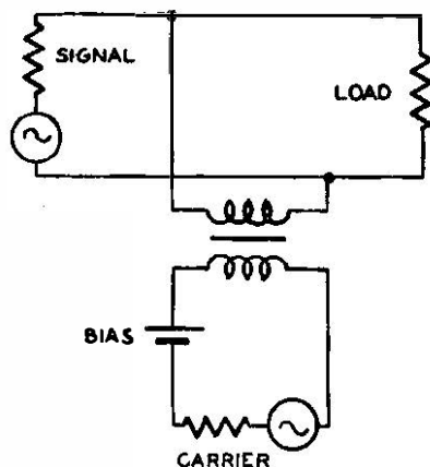
FIG. 3.—UNBALANCED MODULATOR.
