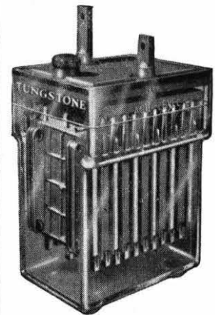
ENCLOSED TYPE CELL
