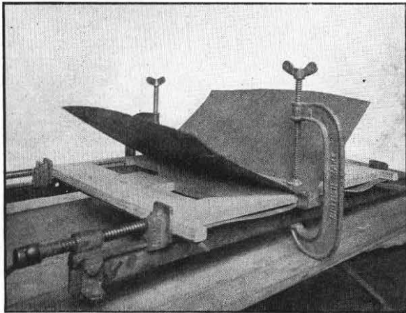
FIG. 2.—EARLY STAGE IN KEYSHELF MANUFACTURE.
