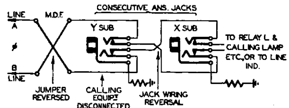
(2) C.B.S. 1 and 2 Non-multiple Exchanges.
