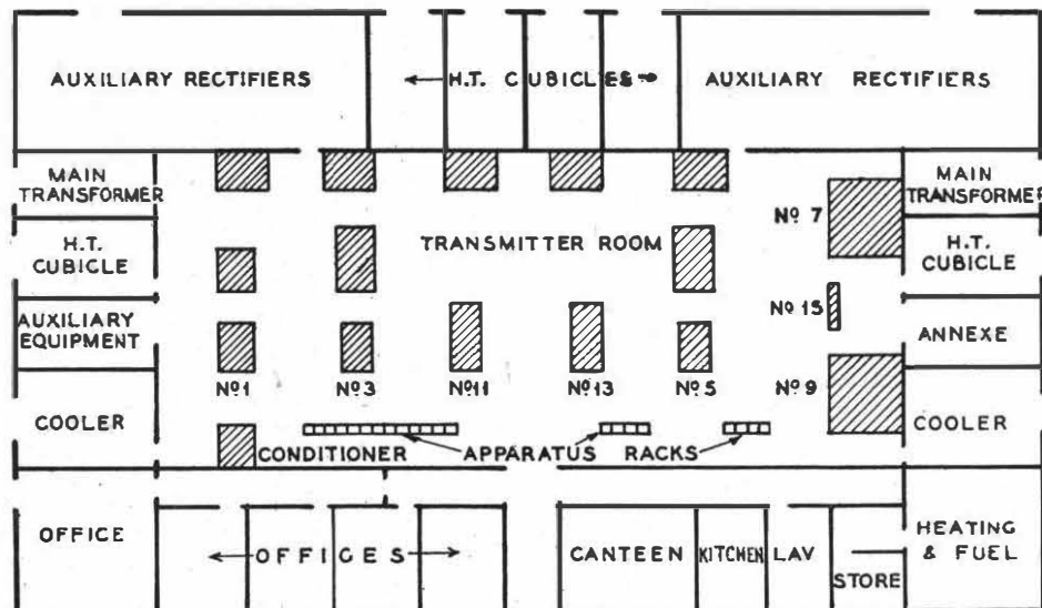
FIG. 7.—LAYOUT OF H.F. TRANSMITTER BUILDING.
