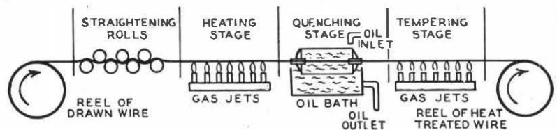
FIG. 1.—HEAT TREATMENT OF CONTINUOUS ROD.
