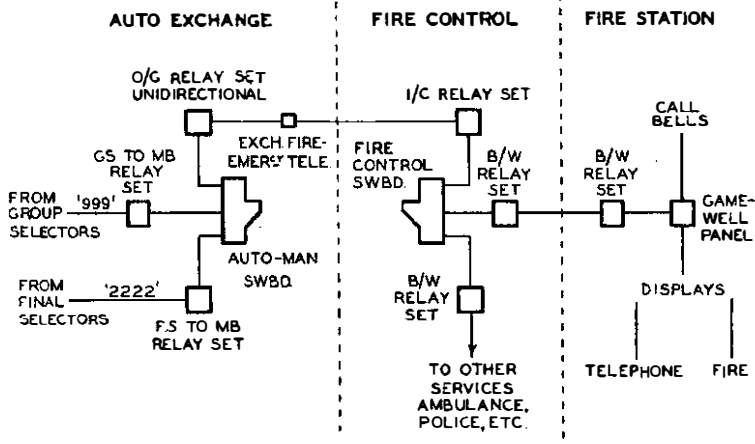
FIG. 3.—OUTLINE OF CIRCUIT ARRANGEMENTS.
