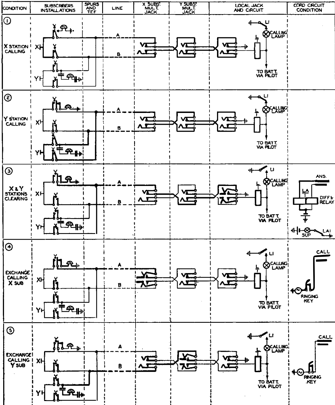
FIG. 3.—CALLING AND CLEARING CONDITIONS FOR C.B.S. 1 INSTALLATION.
