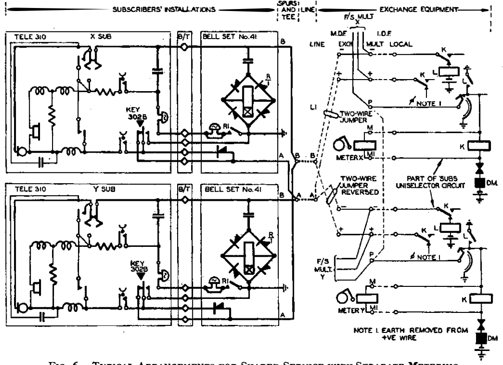
FIG. 6.—TYPICAL ARRANGEMENTS FOR SHARED SERVICE WITH SEPARATE METERING.
