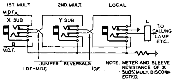
(1) C.B.S. 1 Multiple Exchanges.
