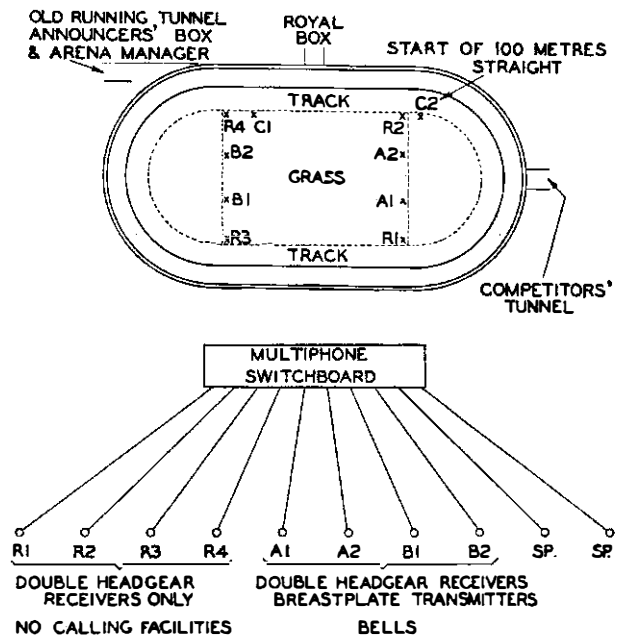
FIG. 5.—FIELD EVENTS NETWORK.
