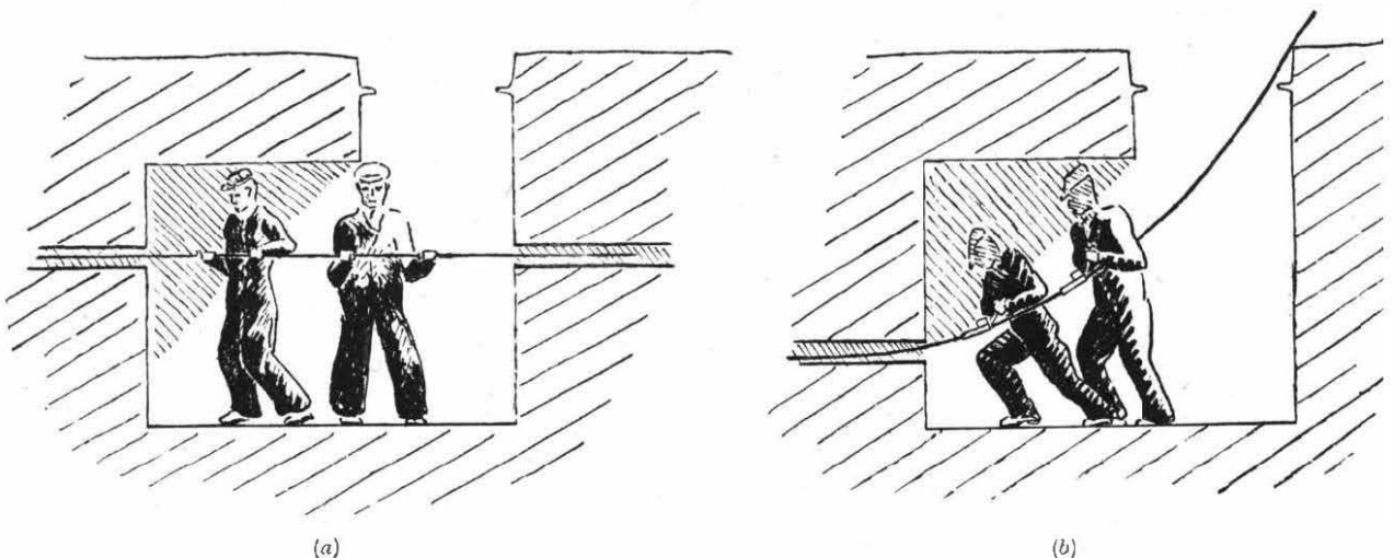
FIG. 8.—(a) RODDING THROUGH A MANHOLE. (b) RODDING WITH THE AID OF HAND-FEEDING GRIPS.
