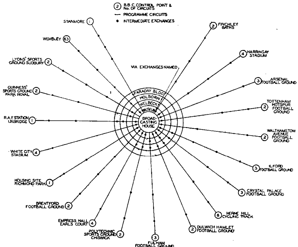
FIG. 2.—B.B.C. PROGRAMME CIRCUITS (NON-AMPLIFIED).
