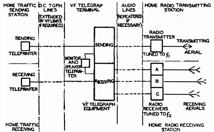
FIG. 3.—LAYOUT OF SINGLE-SIDEBAND RADIO TELEGRAPH SYSTEM.
