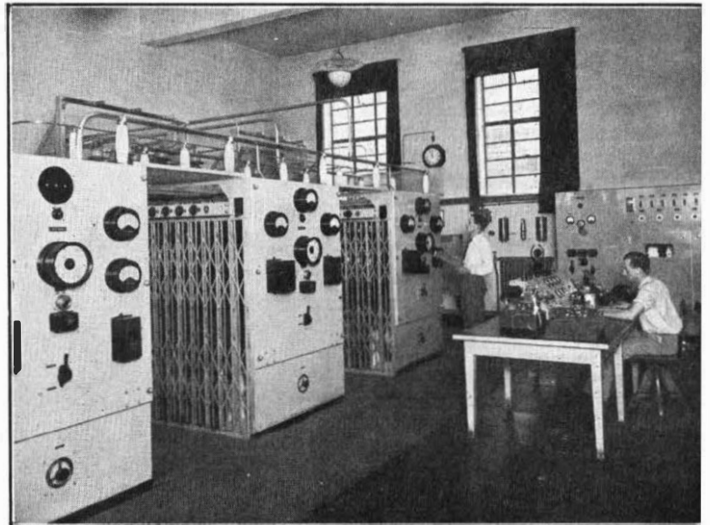
FIG. 5.—HIGH-POWER AMPLIFIER STAGE OF V.L.F. TRANSMITTER.
