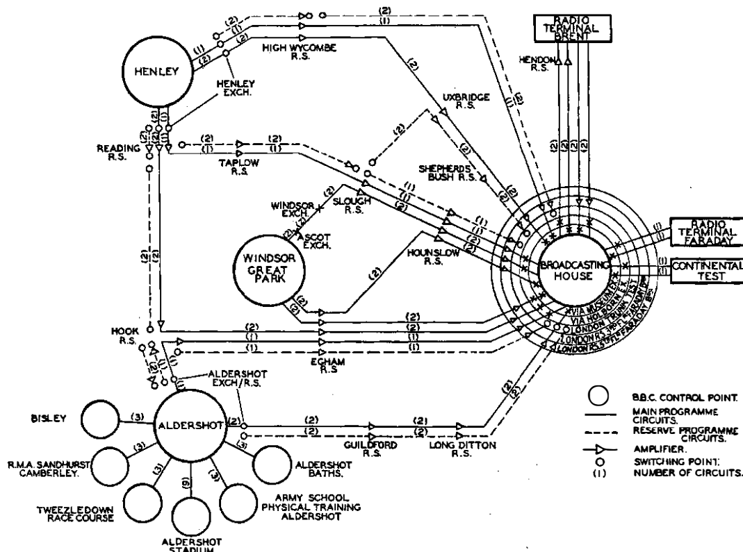
FIG. 3.—B.B.C. PROGRAMME CIRCUITS (AMPLIFIED).
