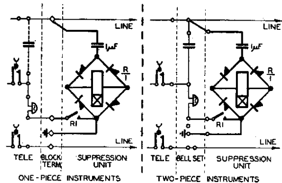
FIG. 4.—TYPICAL ARRANGEMENTS FOR SUPPRESSION OF BELL-TINKLING.
