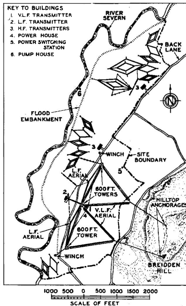
FIG. 1.—PLAN OF SITE.
