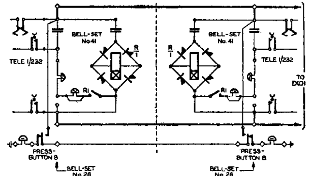
FIG. 8.—SIMPLE PARALLEL EXTENSION FOR USE WHERE EXCHANGE MULTIPLE IS EXHAUSTED.
