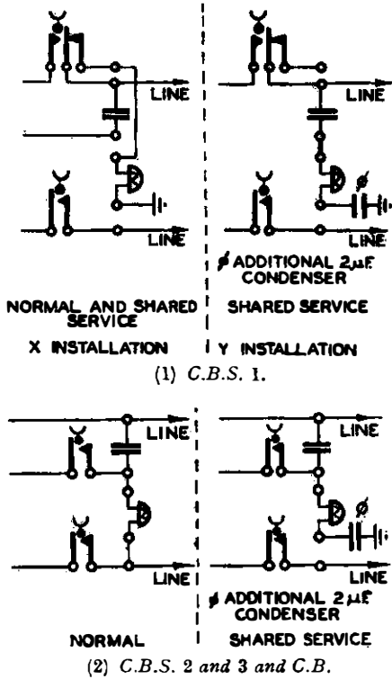
FIG. 1.—MANUAL WORKING—ALTERATIONS AT SUBSCRIBER'S PREMISES.
