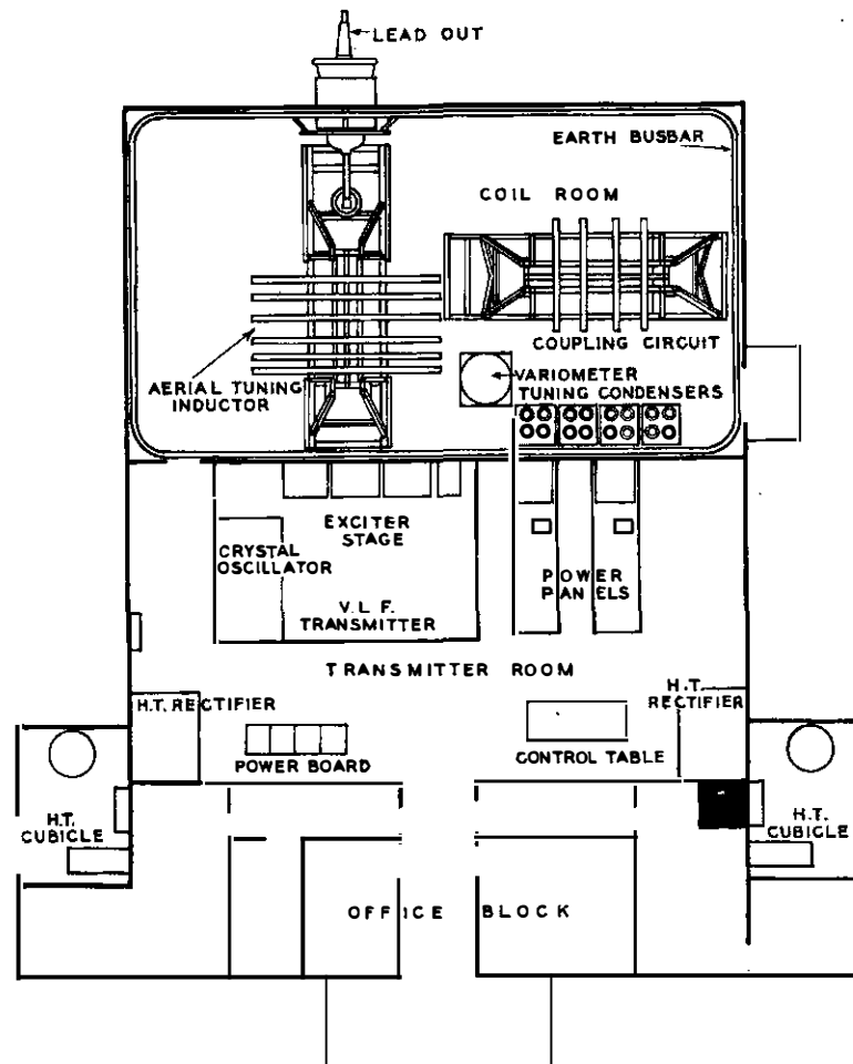
FIG. 4.—LAYOUT OF V.L.F. TRANSMITTER BUILDING.
