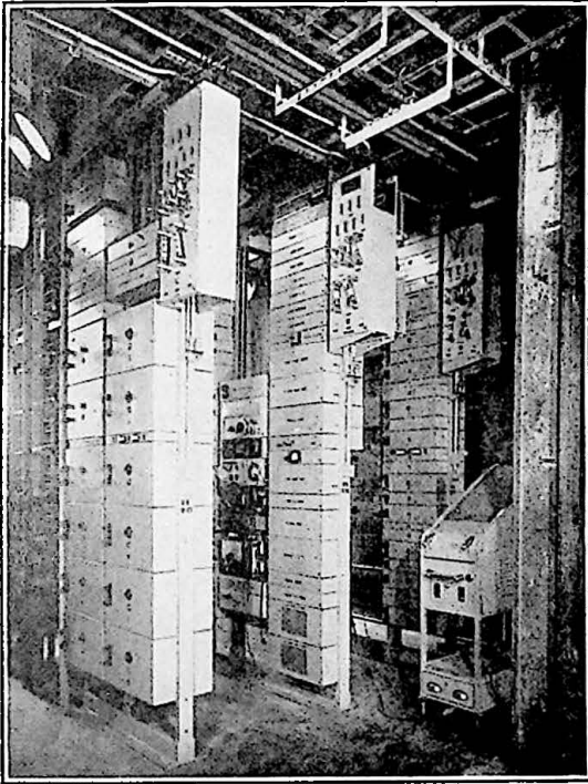
FIG. 4.—12-CHANNEL CARRIER EQUIPMENT INSTALLED IN CALAIS REPEATER STATION.
