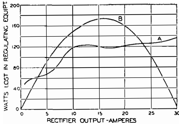
FIG. 9.—LOSSES DUE TO VOLTAGE REGULATION.
