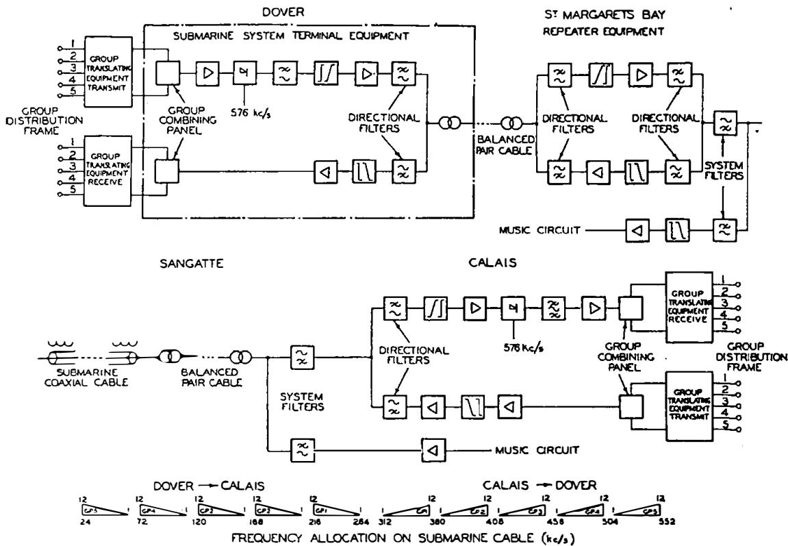
FIG. 1.—BLOCK SCHEMATIC DIAGRAM OF DOVER-CALAIS SUBMARINE SYSTEM.
