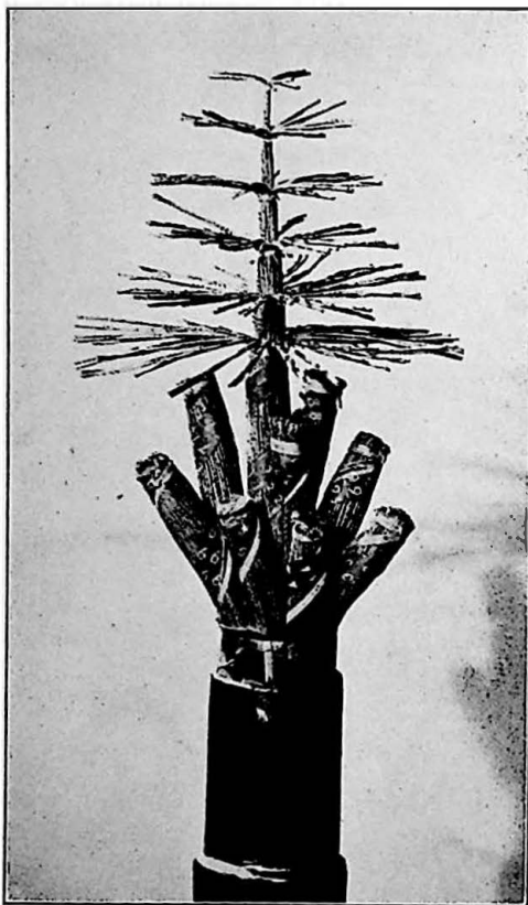
FIG. 5.—CABLE END SHOWING UNIT CONSTRUCTION.
