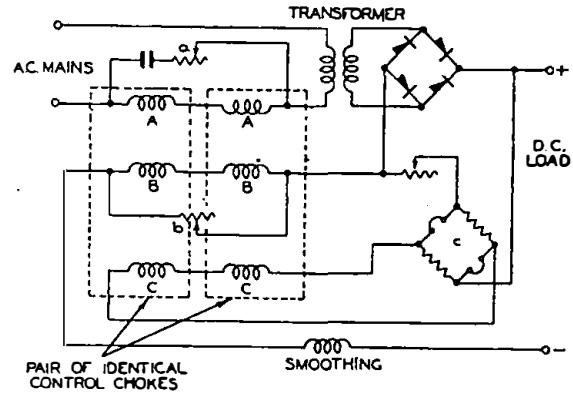
FIG. 4.—TYPICAL CONNECTIONS OF CHOKE WINDINGS.
