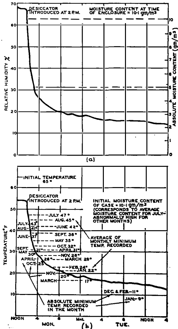
FIG. 2.—EFFECT OF INTRODUCING SILICA-GEL DESICCATORS
