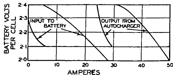
FIG. 8.—AUTOCHARGER FOR BATTERY WITH CONTINUOUS 25A LOAD.
