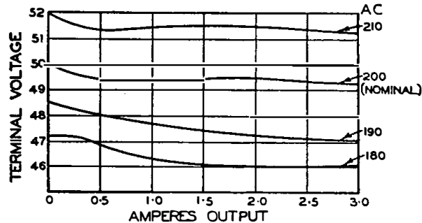
FIG. 5.—MAINS UNIT USED ON V.F. SIGNALLING EQUIPMENT RACK.
