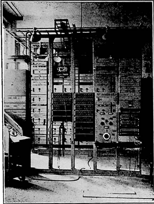
FIG. 6.—12-CHANNEL TERMINAL EQUIPMENT INSTALLED IN PARIS (RUE ST. ANAND) REPEATER STATION.
