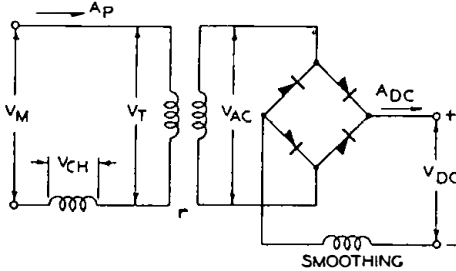
FIG. 2.—SKELETON CIRCUIT OF CHOKE-CONTROLLED RECTIFIER.
