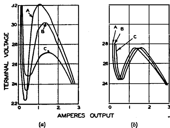
FIG. 6.—AUTOCHARGER OUTPUT CURVES.
