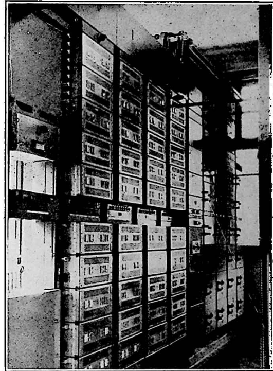
FIG. 5.—BRITISH CARRIER EQUIPMENT INSTALLED ALONGSIDE FRENCH EQUIPMENT IN AMIENS REPEATER STATION.
