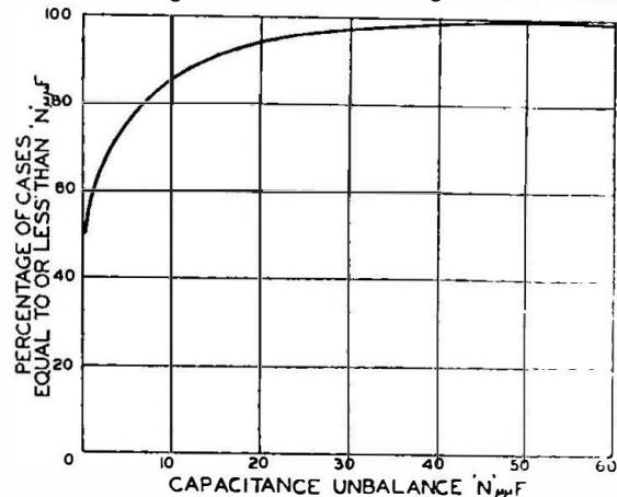
FIG. 6.—DISTRIBUTION OF CAPACITANCE UNBALANCES ON ONE UNIT OF 6½ LB. POST OFFICE TYPE UNIT CABLE. (LENGTH 1 MILE. STRAIGHT JOINTED. 5,050 CASES TESTED.)
