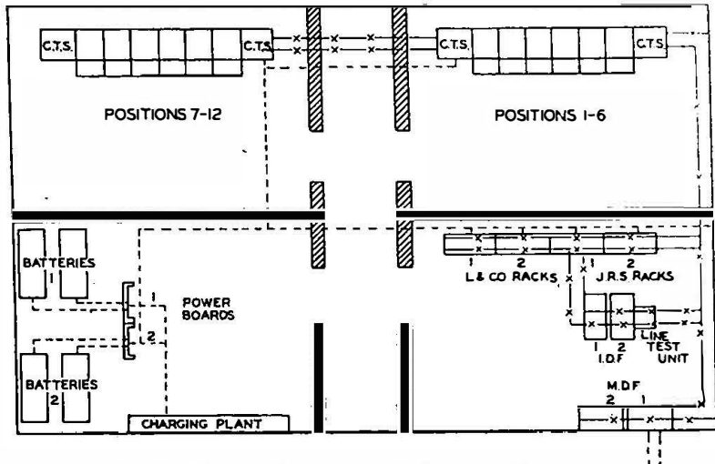
FIG. 2.—TYPICAL LAYOUT FOR 12-POSITION EXCHANGE.
