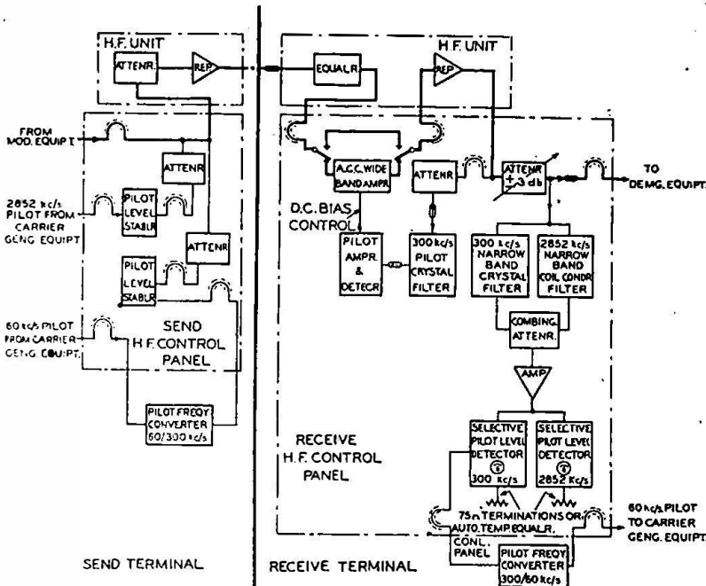
FIG. 2.—BLOCK SCHEMATIC OF H.F. CONTROL PANELS.
