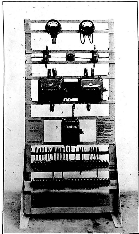
FIG. 8.—POWER BOARD.
