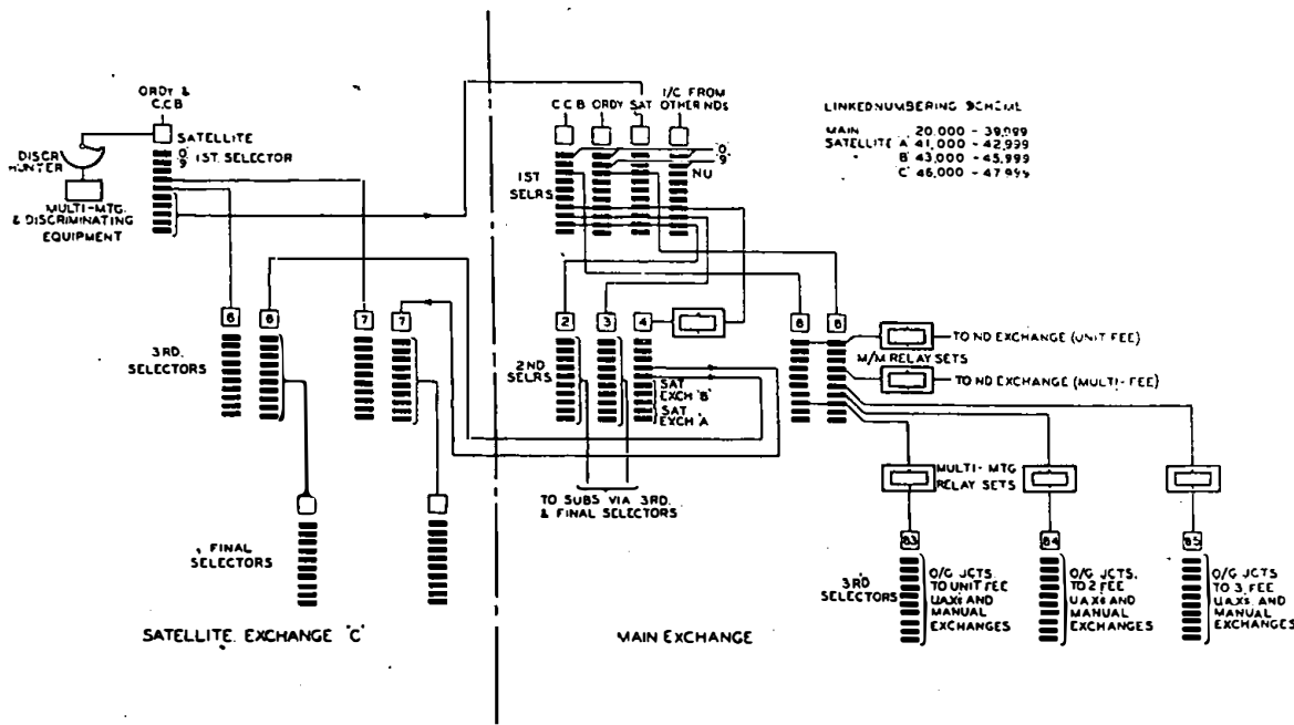
FIG. 1.—TYPICAL TRUNKING ARRANGEMENTS.
