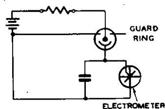
FIG. 4.—CELL USED UNDER D.C. CONDITIONS.
