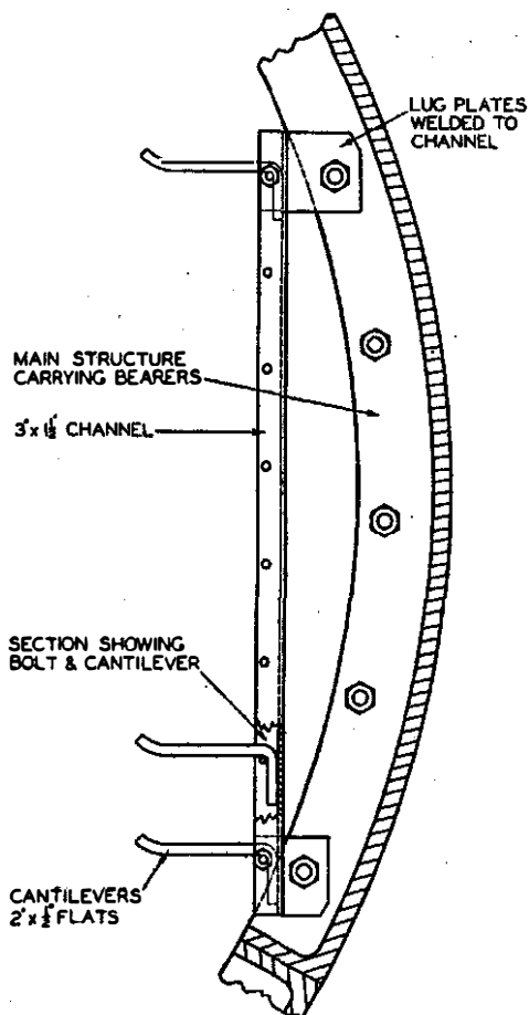
FIG. 4.—CABLE BEARER.
