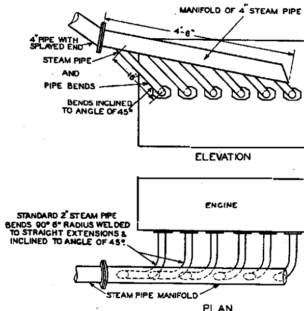
FIG. 5.—FABRICATED EXHAUST-MANIFOLD FOR 67 kW PETROL ELECTRIC SET.
