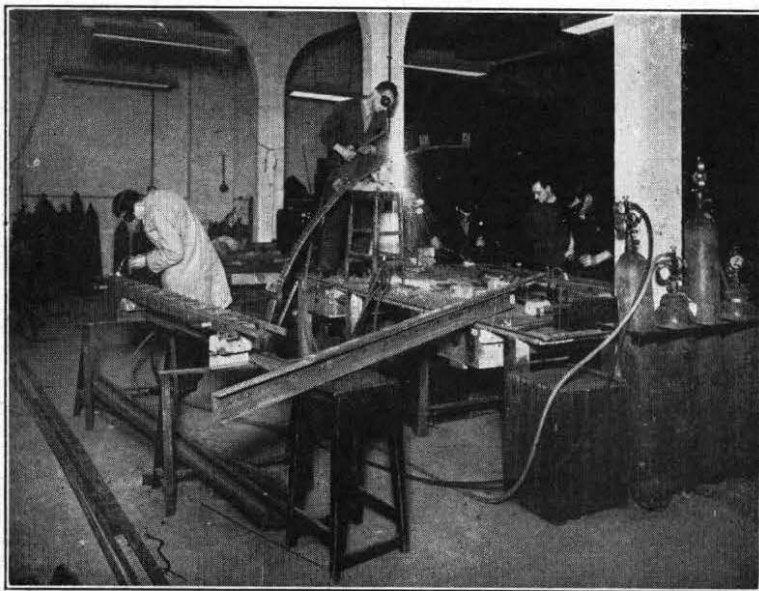
FIG. 3.—WELDER'S BENCH.
