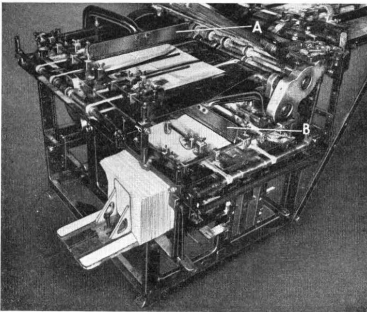
FIG. 8.—FOLDING MACHINE.
