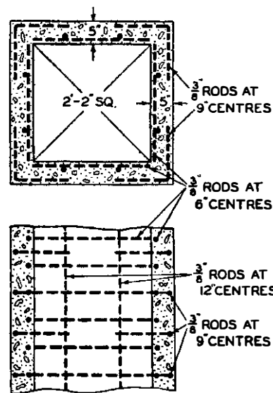
FIG. 7.—REINFORCEMENT OF TYPICAL MANHOLE SHAFT.
