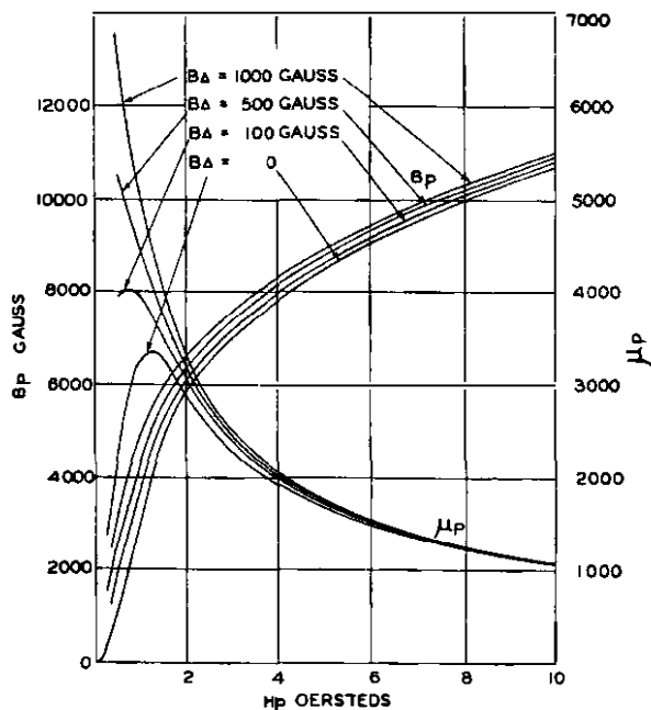
FIG. 4.—MAGNETISATION AND PERMEABILITY CURVES WITH SUPERPOSED ALTERNATING MAGNETISATION.
