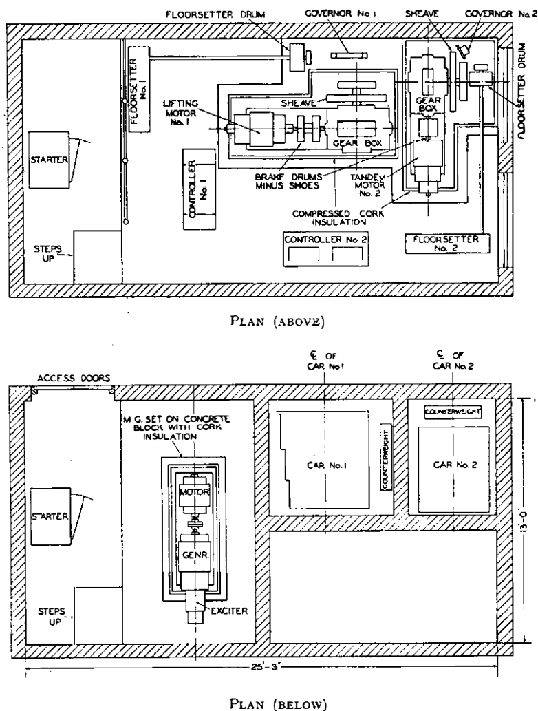
FIG. 7.—LAYOUT OF LIFT MOTOR ROOM.
