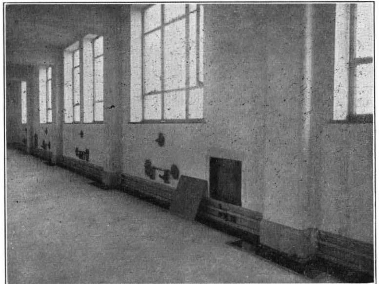
FIG. 2.—STEEL SKIRTING, HEATING PIPE TRENCH AND CONCEALED TELEPHONE SUB-DISTRIBUTION BOARD.
