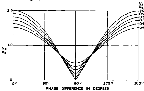
FIG. 4.—VARIATION OF V_D/V_2 .
