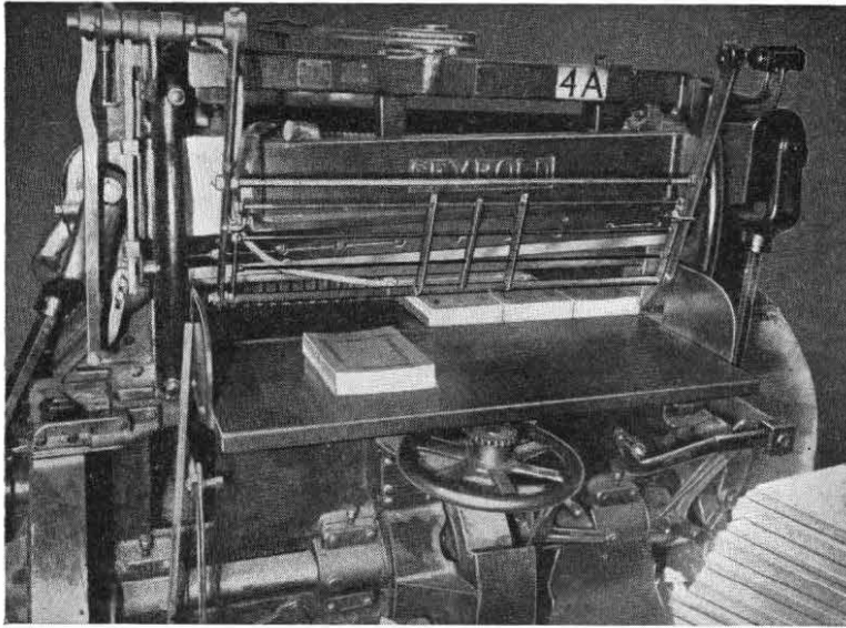
FIG. 10.—THE GUILLOTINE.
