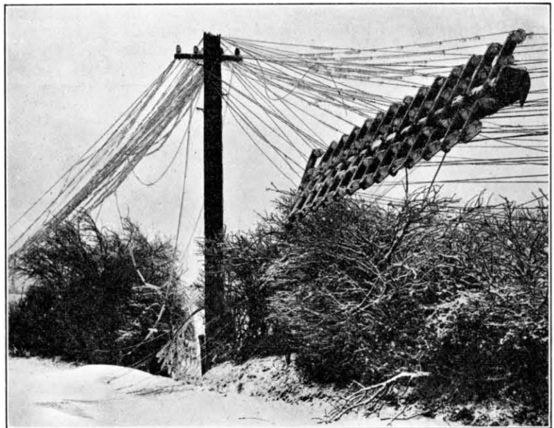
FIG. 8.—BROKEN POLE "SOMEWHERE IN SOMERSET."
