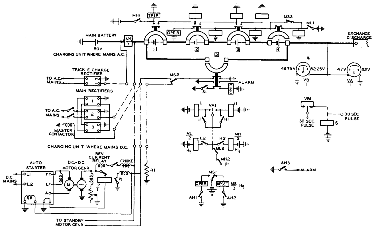
FIG. 9.—CIRCUIT ARRANGEMENTS OF PARALLEL BATTERY AUTOMATIC SYSTEM.
