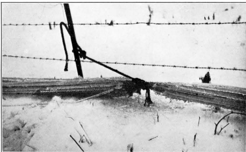
FIG. 5.—FALLEN WIRES FROZEN IN SOLID MASS ON THE OXFORD-WANTAGE ROUTE.
