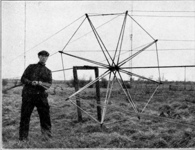
FIG. 2.—NEW SPREADER.
