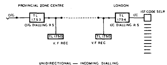
FIG. 1.—METHOD OF WORKING.
