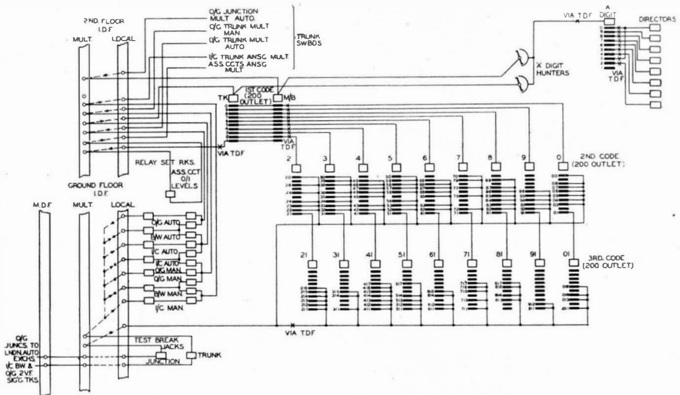
FIG. 3.—TRUNKING DIAGRAM.
