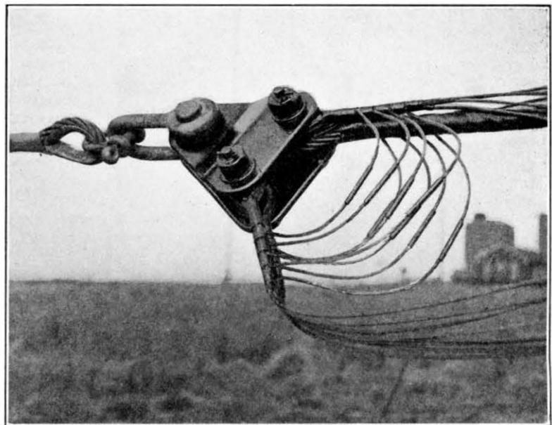
FIG. 3.—TRIANGULAR COUPLING FOR LINKING ADJACENT SPANS.
