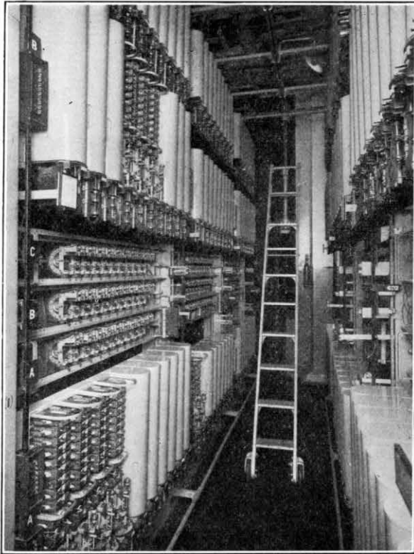
FIG. 5.—TRUNK 1ST CODE SELECTORS.
