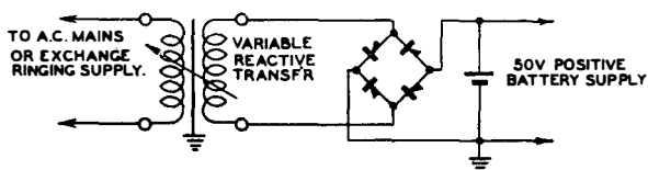
FIG. 7.—50V POSITIVE BATTERY SUPPLY CIRCUIT.
