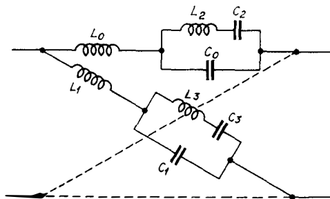
FIG. 3.—FILTER SECTION.
