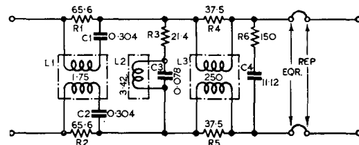
FIG. 7.—TYPICAL EQUALISER CIRCUIT.
