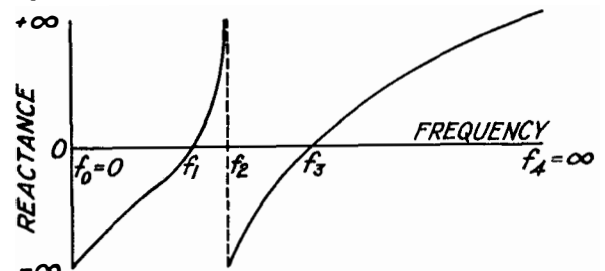
FIG. 10.—REACTANCE-FREQUENCY CHARACTERISTIC.
