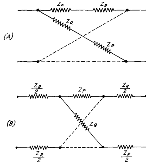
FIG. 4.—EQUIVALENT NETWORKS.
