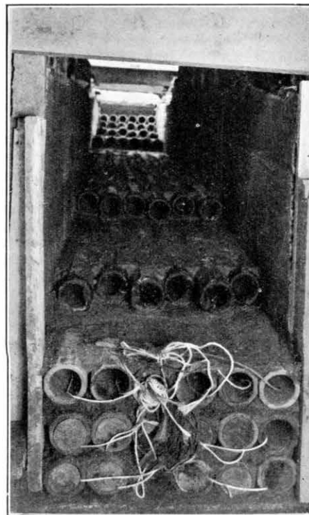
FIG. 2.—DUCT LAYING IN TUNNEL UNDER PARK LANE.
