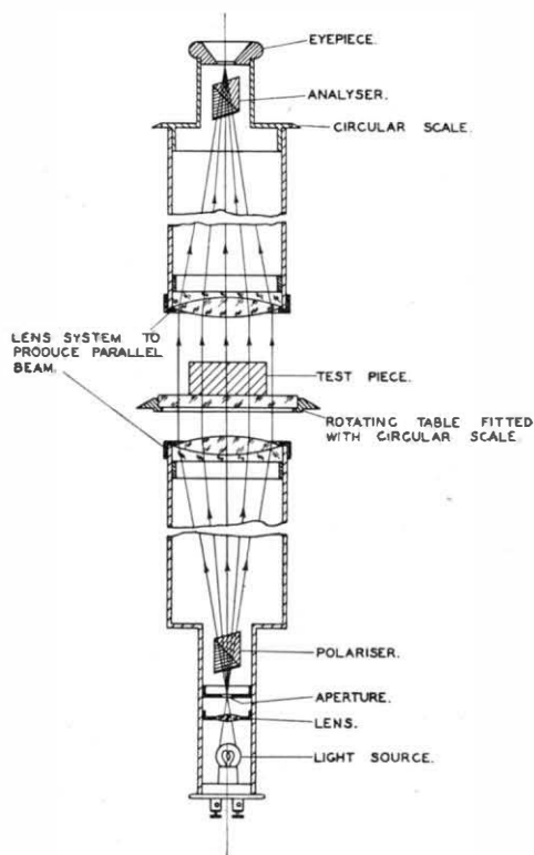
FIG. 10.—POLARISCOPE.
