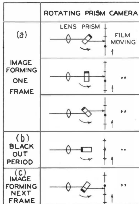
FIG. 4.—OPTICAL PRINCIPLE OF ROTATING PRISM CINEMATOGRAPH CAMERA.
