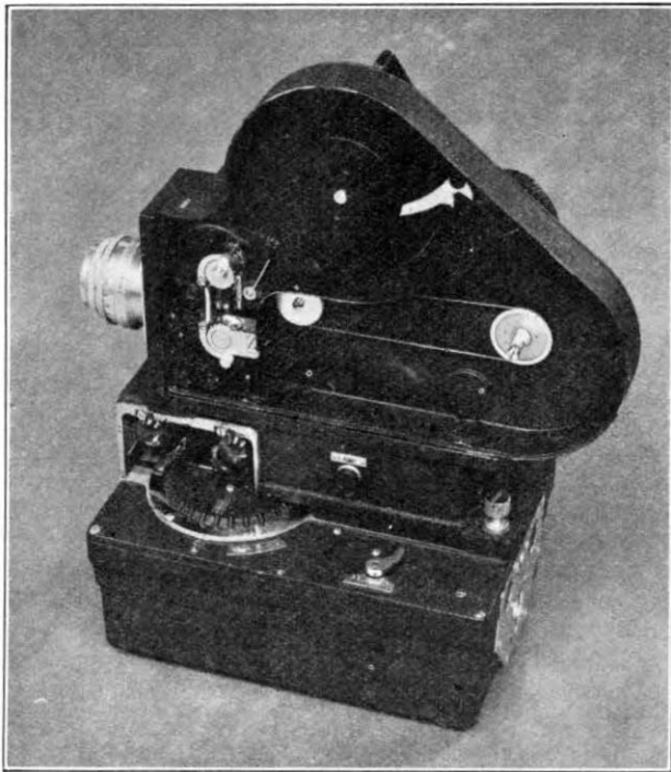
FIG. 3.—WESTERN ELECTRIC 16 MM. HIGH SPEED CAMERA.
