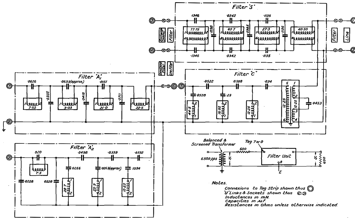
FIG. 6.—FILTERS.
