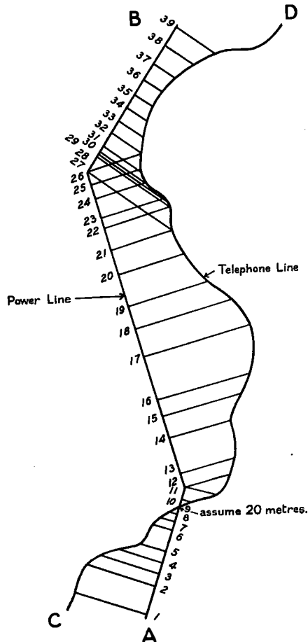
FIG. 6.—PARALLELISM BETWEEN POWER AND TELEPHONE LINES.
