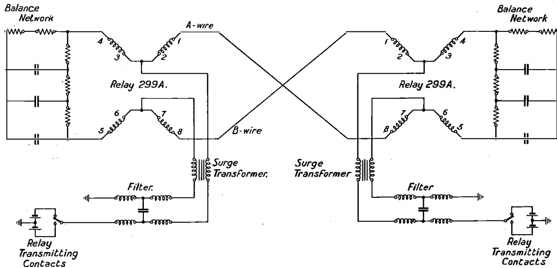
FIG. 2.—CROSSED DUPLEX.
