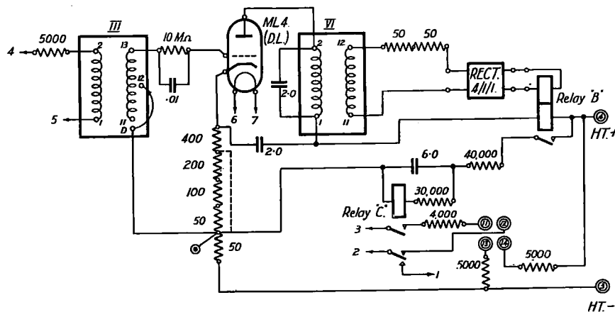
Connexions to Tag Strip shown thus ⊙ Connexions to Modulator - Demodulator Equipment shown thus → 1,2.....7. Testing Point shown thus ⊙ Resistances in Ohms unless otherwise indicated. Capacities in μF.
