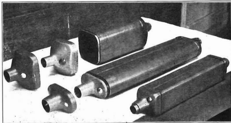
FIG. 7.—DETAILS OF SIEMENS TYPE OF LEAD-COVERED LOADING UNITS.
