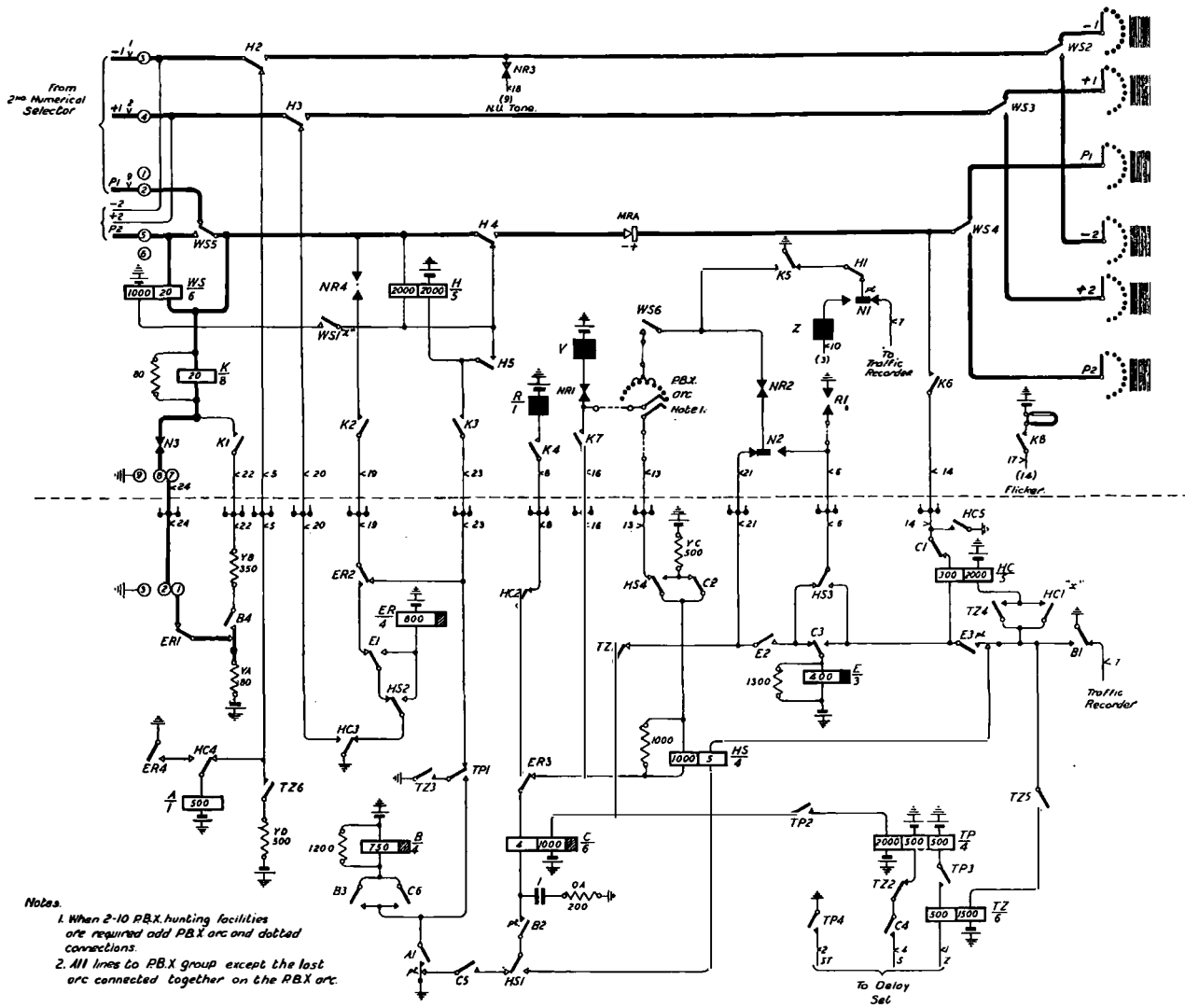
FIG. 7.—COMMON CONTROLLED 200-LINE FINAL SELECTOR.
