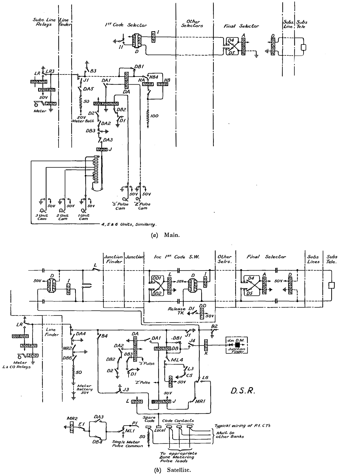
FIG. 6.—SCHEMATIC DIAGRAM OF METERING ARRANGEMENTS.
