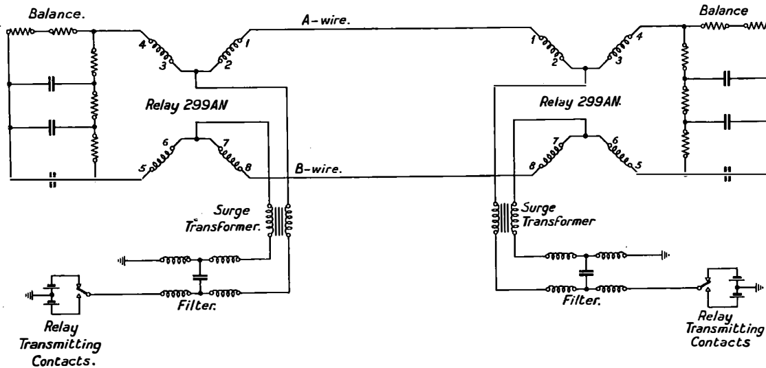
FIG. 1.—DIFFERENTIAL DUPLEX.
