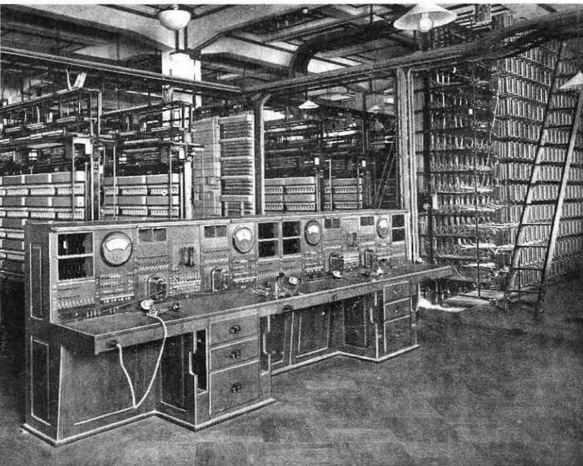
Singapore Automatic Exchange, capacity 9,300 lines.
