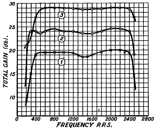
Curve 1—Down to Up Station; Input Transformer tap 12, Receiver Input 1—10 Step Up. Curve 2—As Curve 1, but Receiver Input 1—20 Step Up. Curve 3—Up to Down Station; Input Transformer tap 12, Receiver Input 1—20 Step Up.
