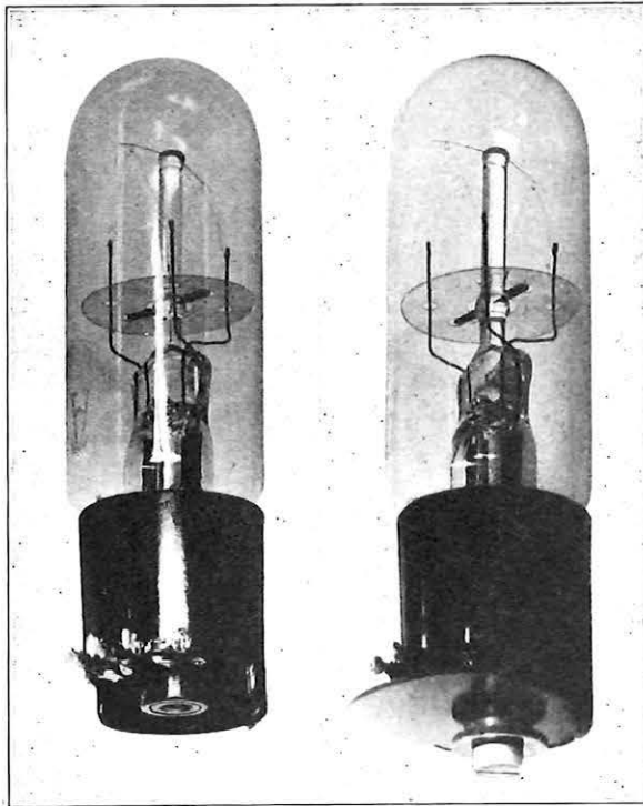
FIG. 7.—100 MA TWIN FILAMENT BALLAST RESISTANCE, SHOWING CONNECTING TAGS, INSULATING WASHER, AND FIXING SCREW.
