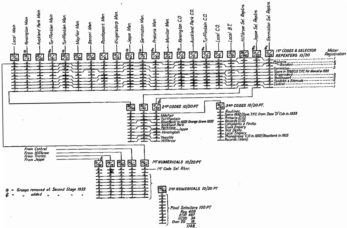
FIG. 2.—TRUNKING DIAGRAM FOR CITY EXCHANGE, 1932/33.
