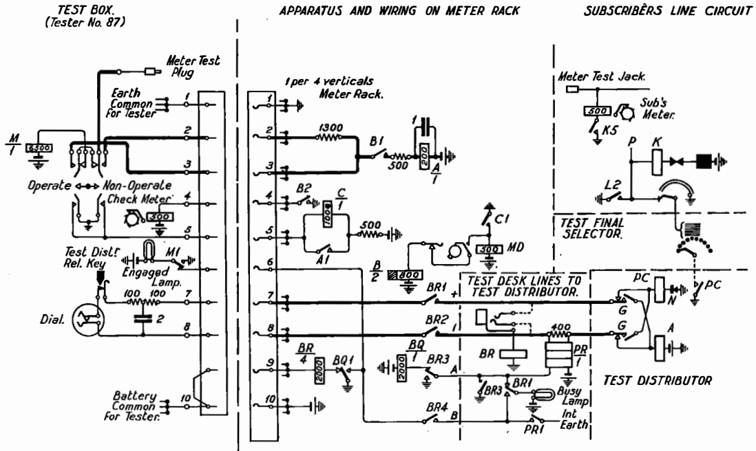
FIG. 1.—ROUTINE TEST CIRCUIT FOR TESTING SUBSCRIBERS' METERS.
