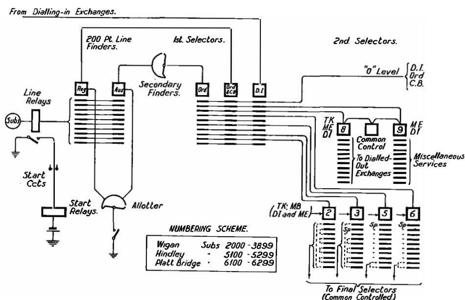
FIG. 1.—TRUNKING DIAGRAM.
