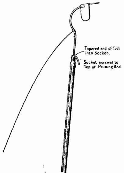
FIG. 1.—WIRE STRINGING TOOL.
