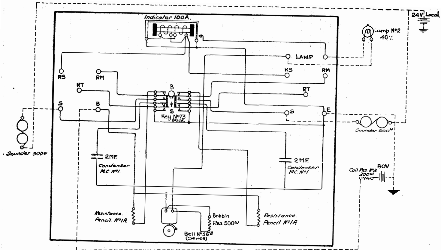
FIG. 2.—WIRING OF ALARM, REPEATER, NO. 3.
