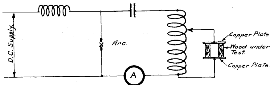
FIG. 1.—TESTING CIRCUIT.
