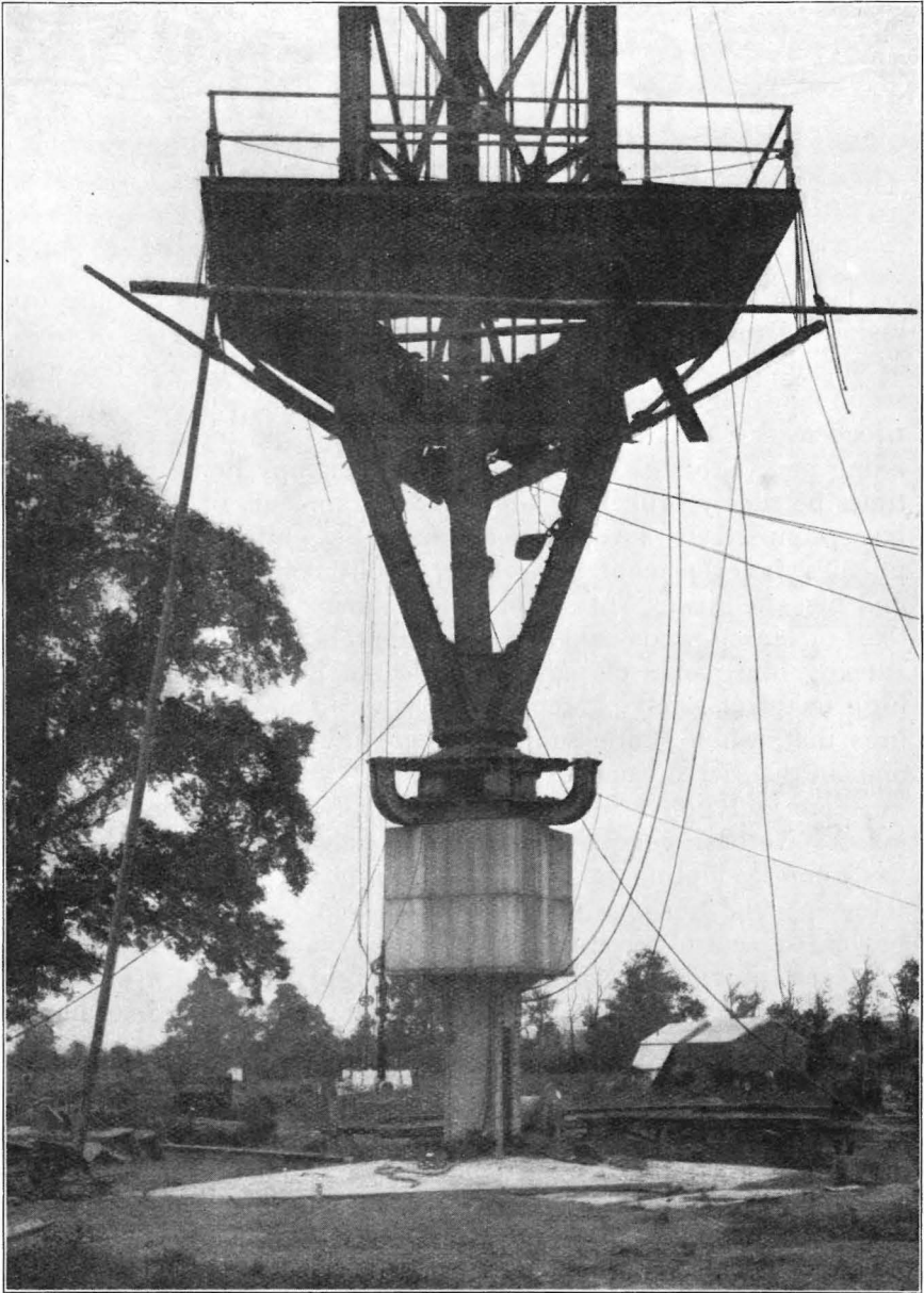
FIG. 1.—BASE OF MAST, SHOWING STEEL STANCHION, GRANITE BLOCKS, PORCELAIN INSULATORS AND BALL SOCKET.
