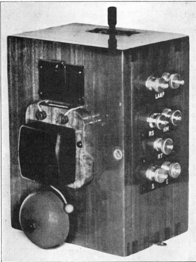
FIG. 1.—ALARM, REPEATER, NO. 3.
