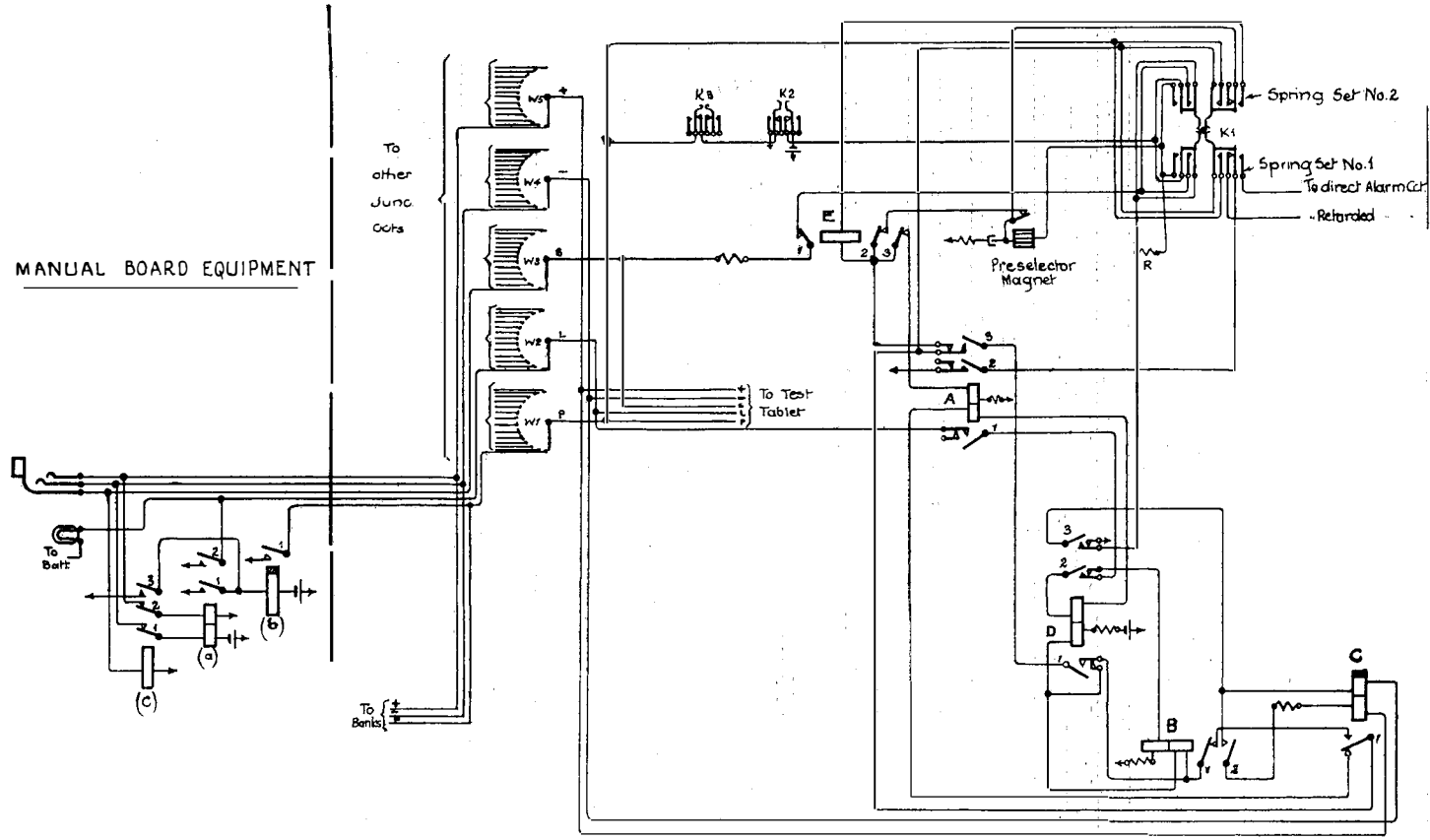
FIG. 1.—AUTO TO MANUAL JUNCTION CIRCUITS. Relay equipment, etc., for routine testing when Circuits are wholly internal.
