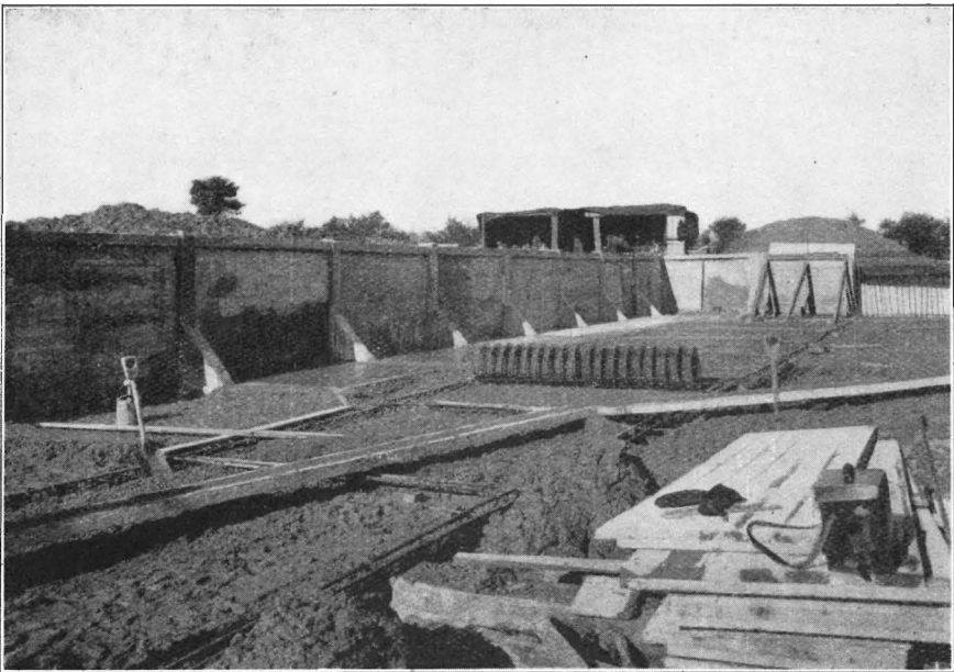
FIG. 2.—500,000 GALLON FERRO-CONCRETE RESERVOIR IN COURSE OF CONSTRUCTION.
