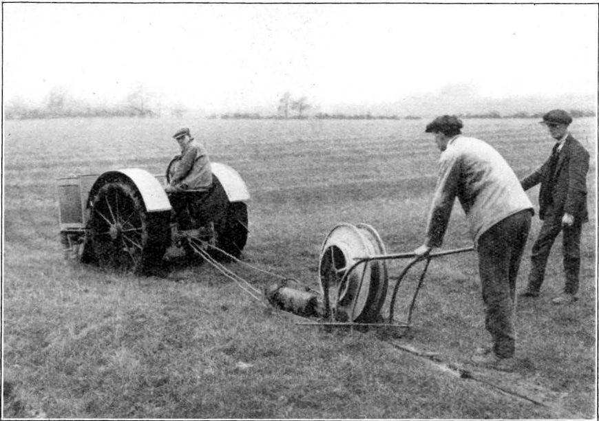
FIG. 4.—WIRE-LAYING PLOUGH.
