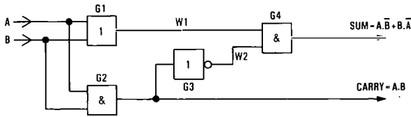
FIG. 2—Diagram of simple half-adder circuit
