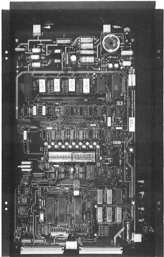
FIG. 8—Control Card 1A
