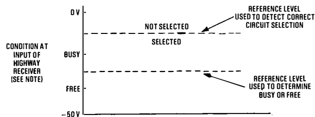
FIG. 4—Use of the selectable reference levels provided in FMTR analogue highway receivers
