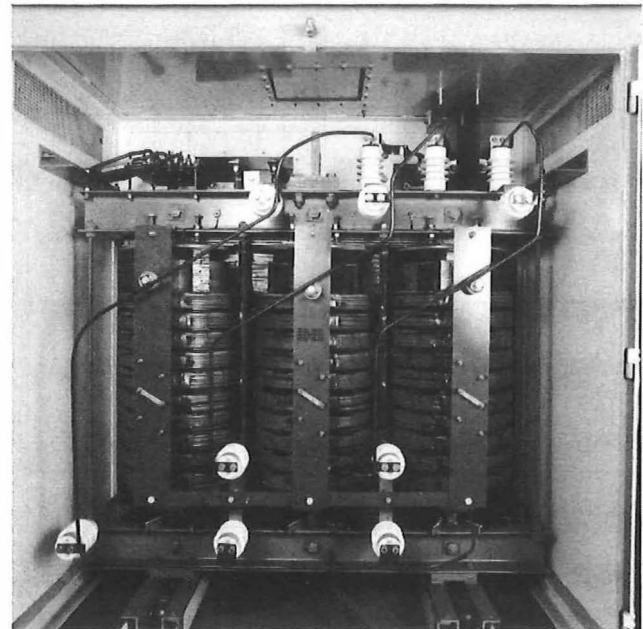
FIG. 6—Interior of transformer cabinet
