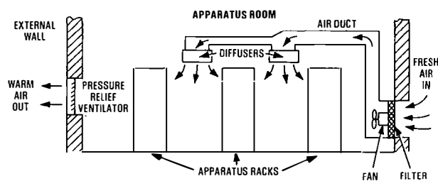
FIG. 1—Exchange cooling system using fresh air and old-style air distribution system
