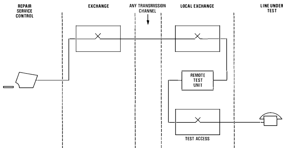
FIG. 1—Remote testing system with dial-up over the PSTN
