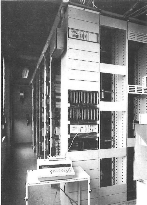
FIG. 1—FMTR traffic recorder (TR8)
