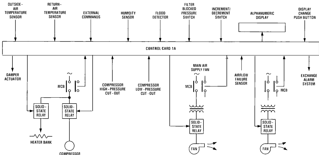
FIG. 9—Simplified control diagram
