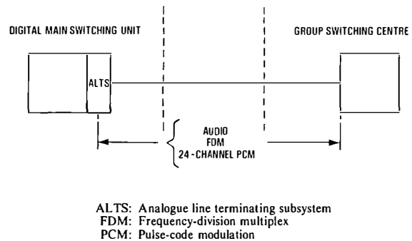
FIG. 2—A/DI circuit analogue presented at the DMSU
