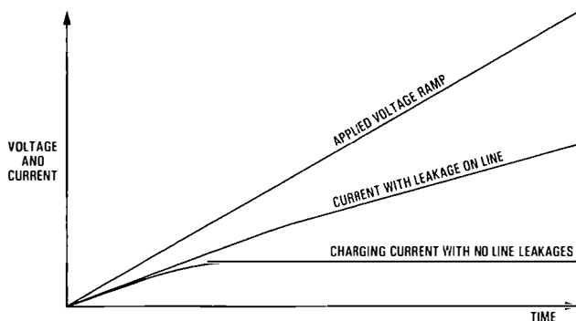
FIG. 9—Capacitance measurement techniques—voltage ramp/ currents graphs
