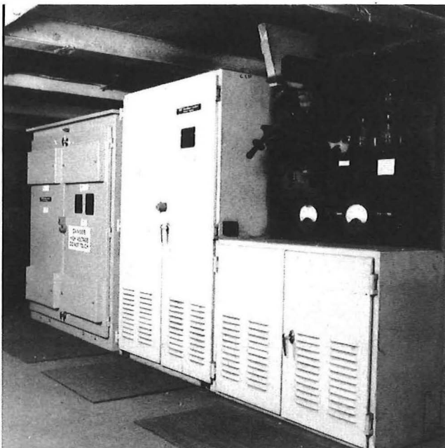
Note: The new transformer cabinet is on the left. The existing rectifier cubicle used to house the new silicon rectifiers is in the centre, and to the right is the DC switchgear
