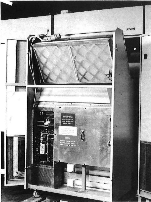
FIG. 3—BT standard cooling unit
