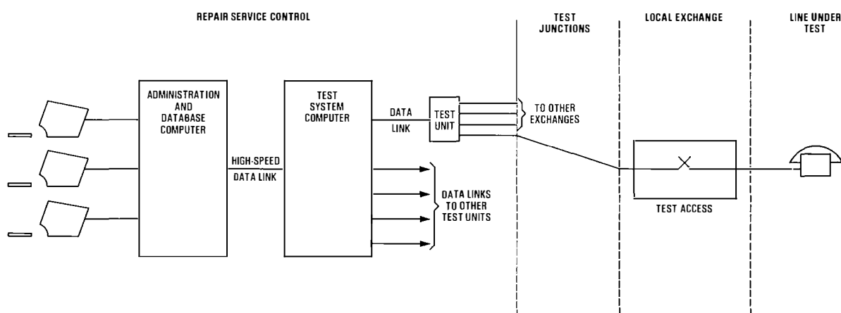
FIG. 2—Test system with integrated database
