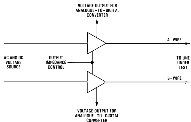
FIG. 10—Block diagram of a test unit designed to locate faults
