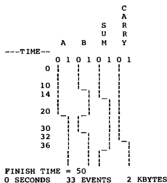
FIG. 5—Graphic output from simulation of HALFADDER
