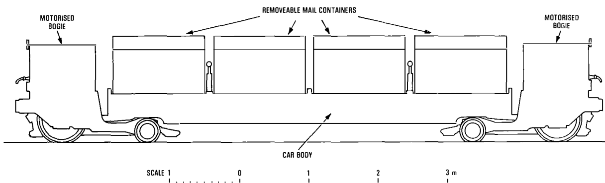
FIG. 3—Rolling stock layout
