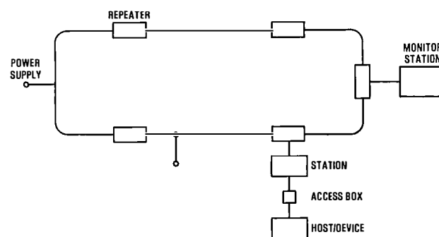
The Cambridge Ring
