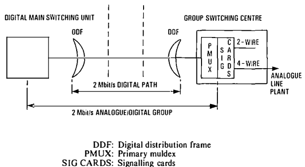
FIG. 3—A/DI circuit digitally presented at the DMSU
