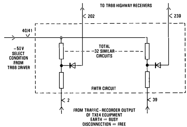
(a) FMTR analogue circuit access provided on plug-in units installed in exchange equipment racks
