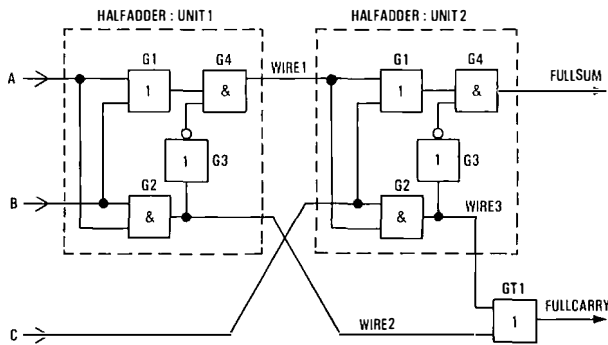
FIG. 6—Diagram of full-adder circuit, built up from 2 half adders
