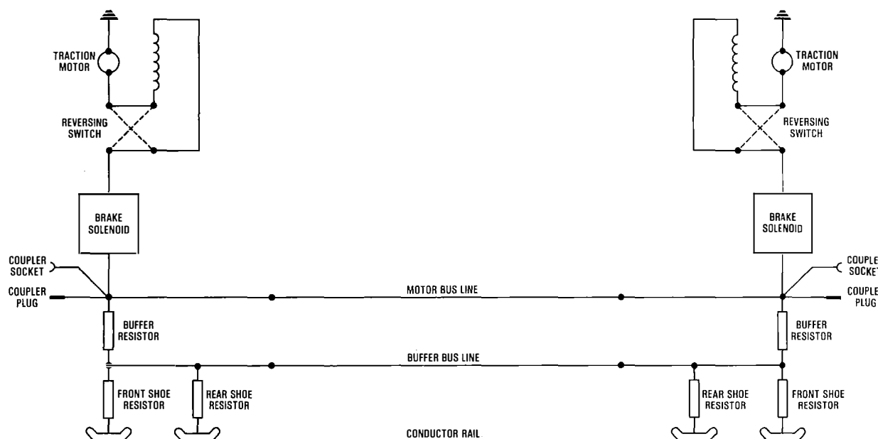
FIG. 4—Rolling stock circuit diagram
