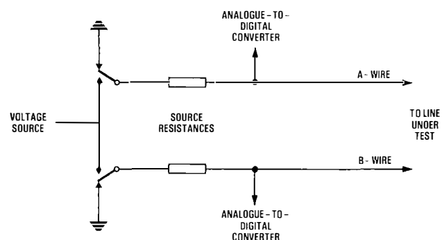
FIG. 8—Block diagram of a unit suitable for testing over junctions
