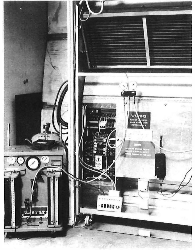
FIG. 4—Charging the Cooling Unit 1A/15 kW with refrigerant gas at the manufacturers works
