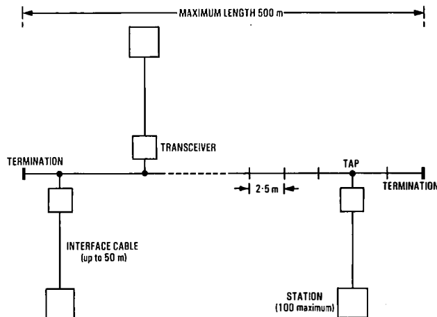
A single-segment Ethernet configuration
