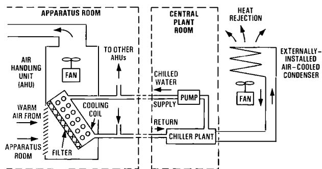
FIG. 2—Exchange cooling system using a central water-cooling plant
