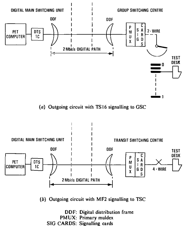
Fig. 4—Testing arrangements for outgoing circuits from a DMSU
