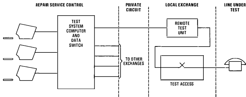
FIG. 3—Test system designed to locate faults
