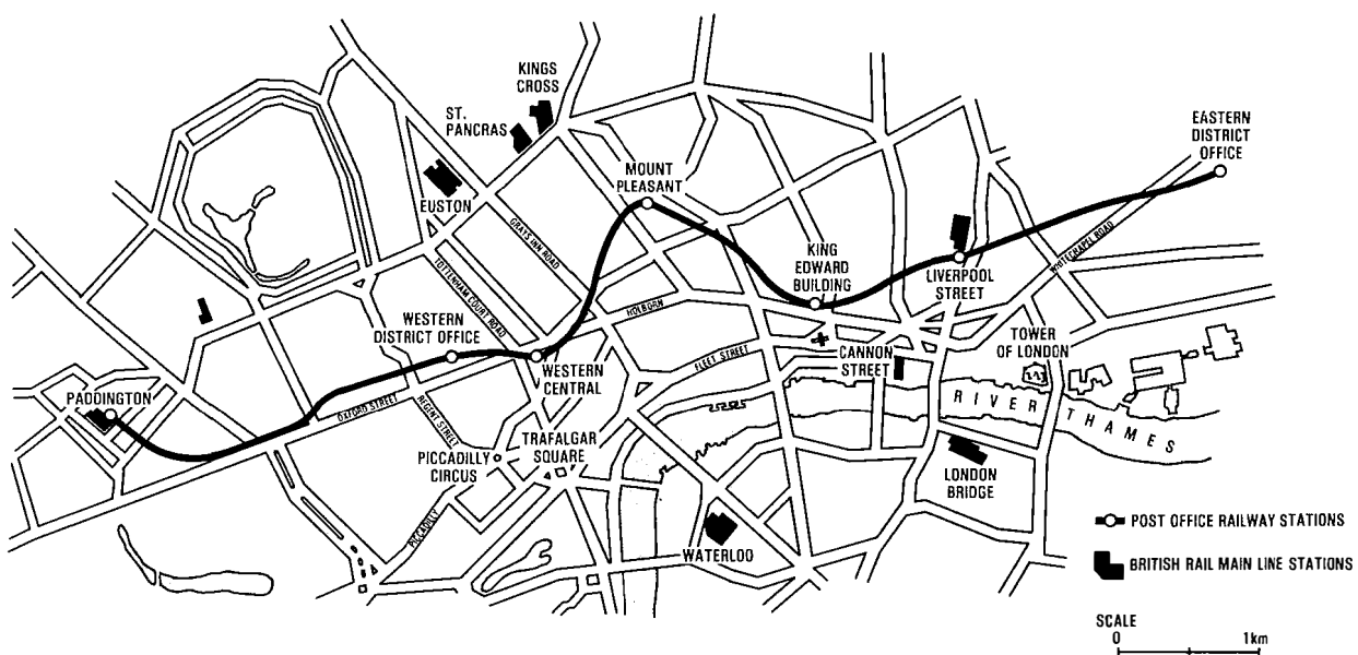
FIG. 1—Post Office Railway
