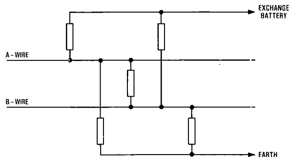
FIG. 5—Possible line leakage paths
