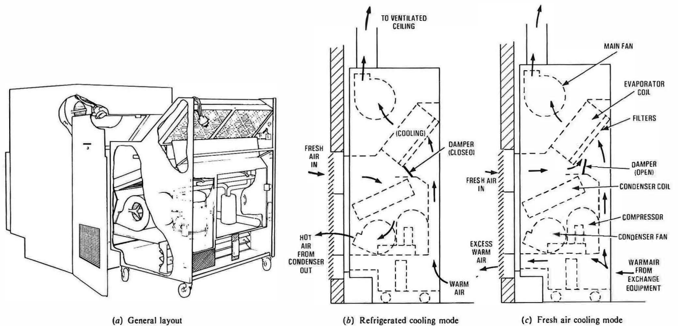
FIG. 5—Operation of standard cooling unit
