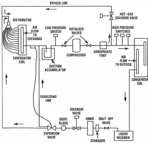
FIG. 6—Refrigeration arrangements of the BT standard cooling unit
