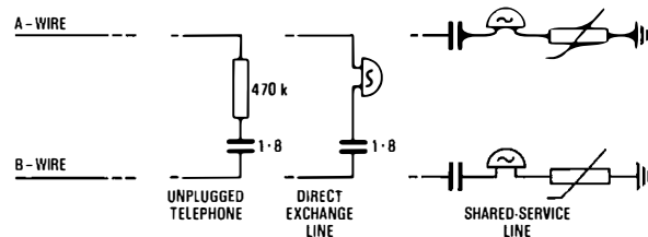
FIG. 6—Commonly found terminations
