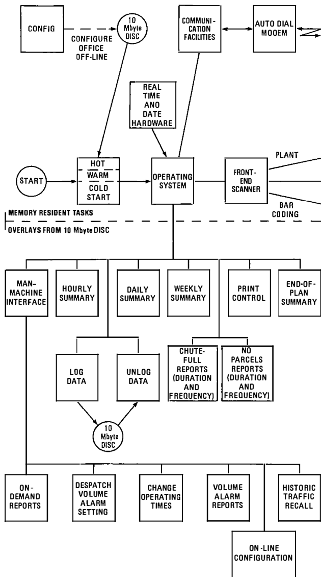
FIG. 3—Block diagram of TRIPOS software task organisation
