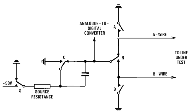
FIG. 7—Block diagram of remote testing unit
