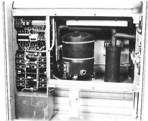
FIG. 7—Compressor unit
