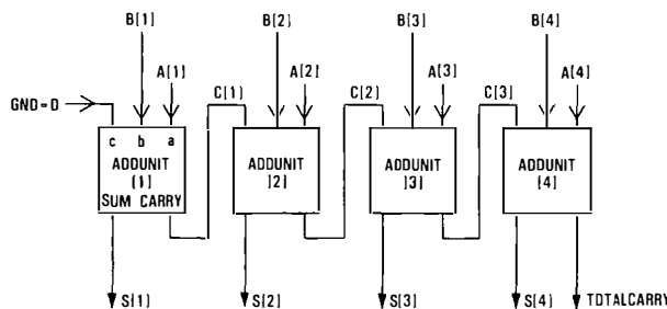
FIG. 8—Diagram of 4 bit binary parallel adder, built up from 4 binary full adders
