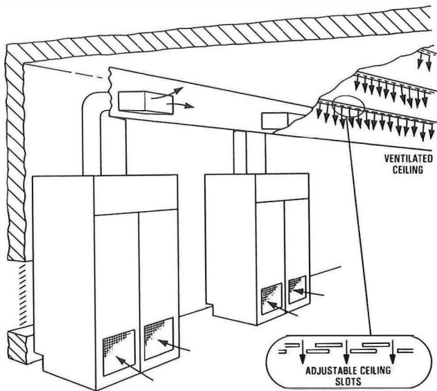
FIG. 10—Common ventilated-ceiling system
