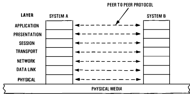
The reference model for open systems interconnection
