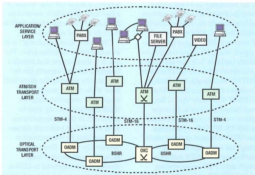
Figure 19—METON demonstrator outline in the Stockholm Gigabit Network
