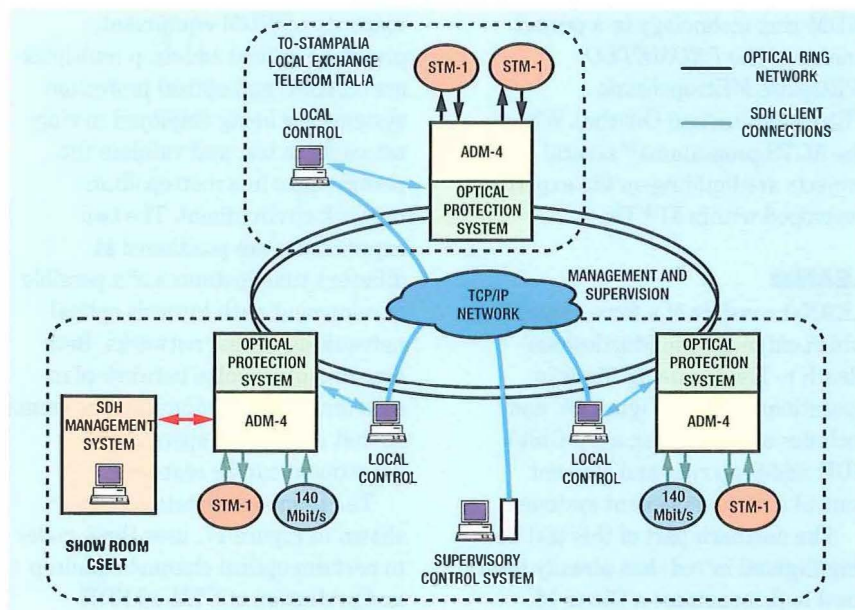
Figure 18—PROMETEO optical bidirectional self-healing ring in Turin metropolitan network
