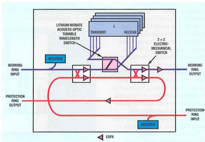
Figure 6 – Wavelength add-drop node
