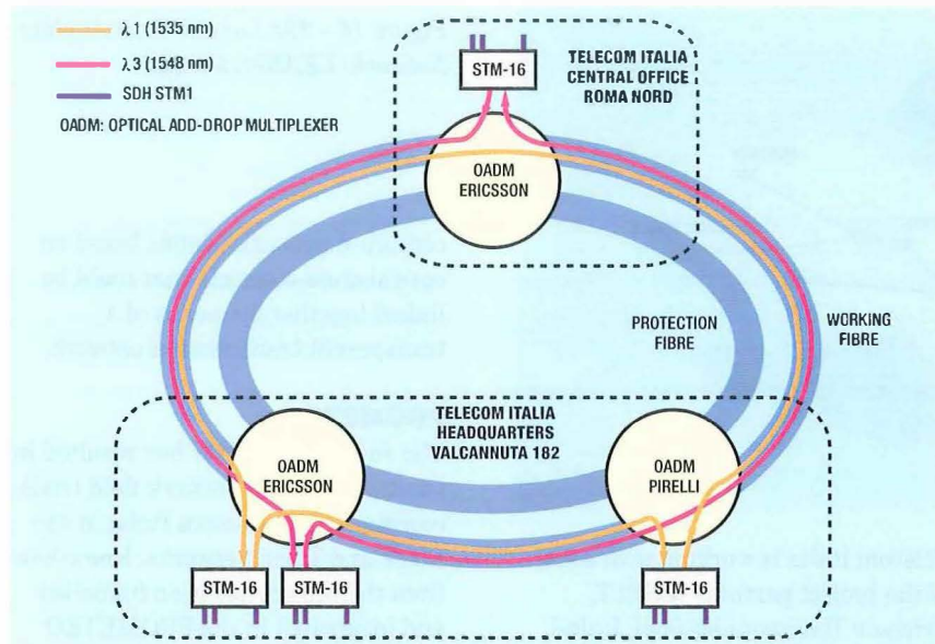
Figure 17—PROMETEO optical unidirectional self-healing ring in the Rome metropolitan network
