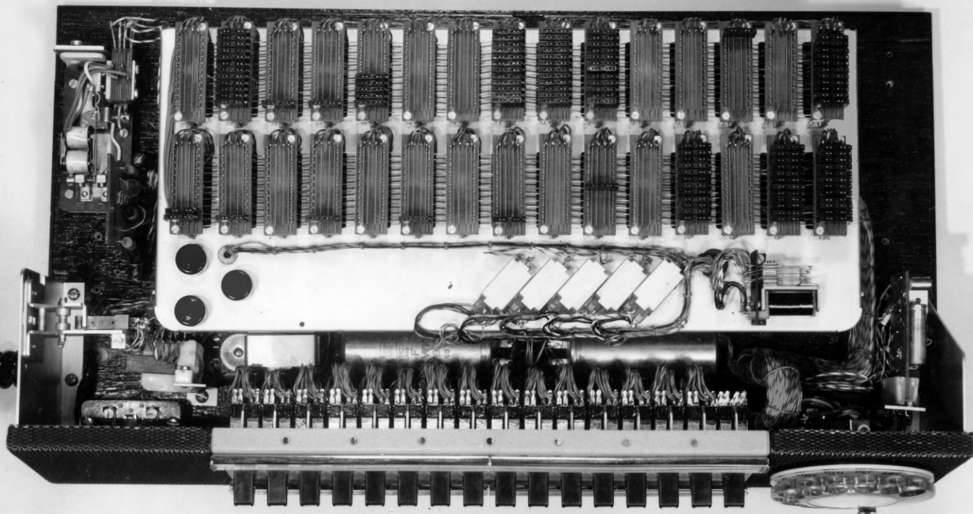
REPETEL 1 ST PROTOTYPE PLAN VIEW SHOWING TRANSLATORS
