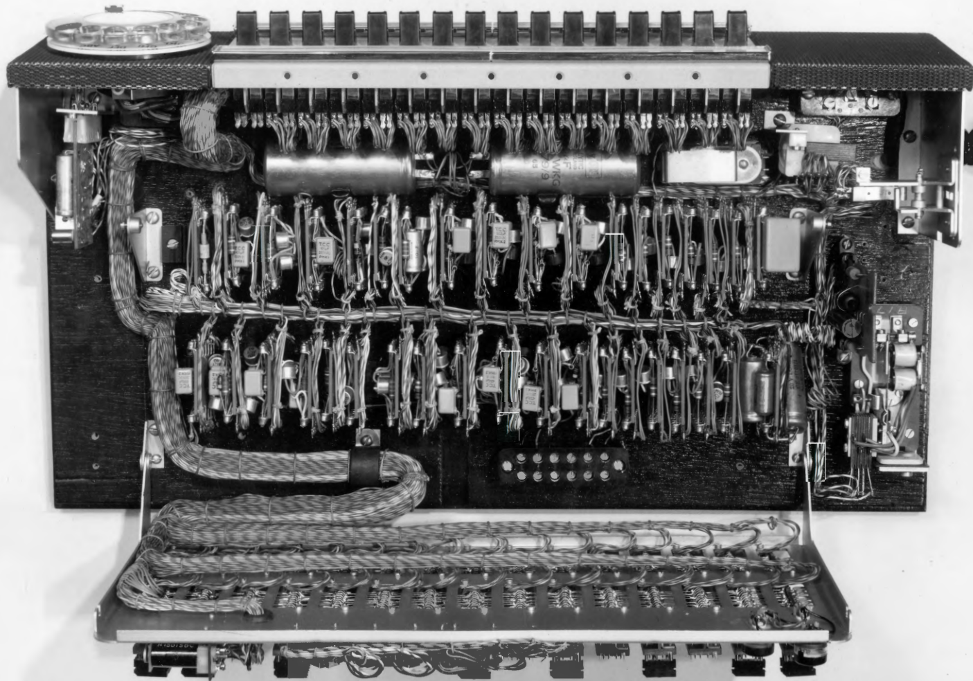
REPETEL 1 ST PROTOTYPE PLAN VIEW SHOWING MODULES
